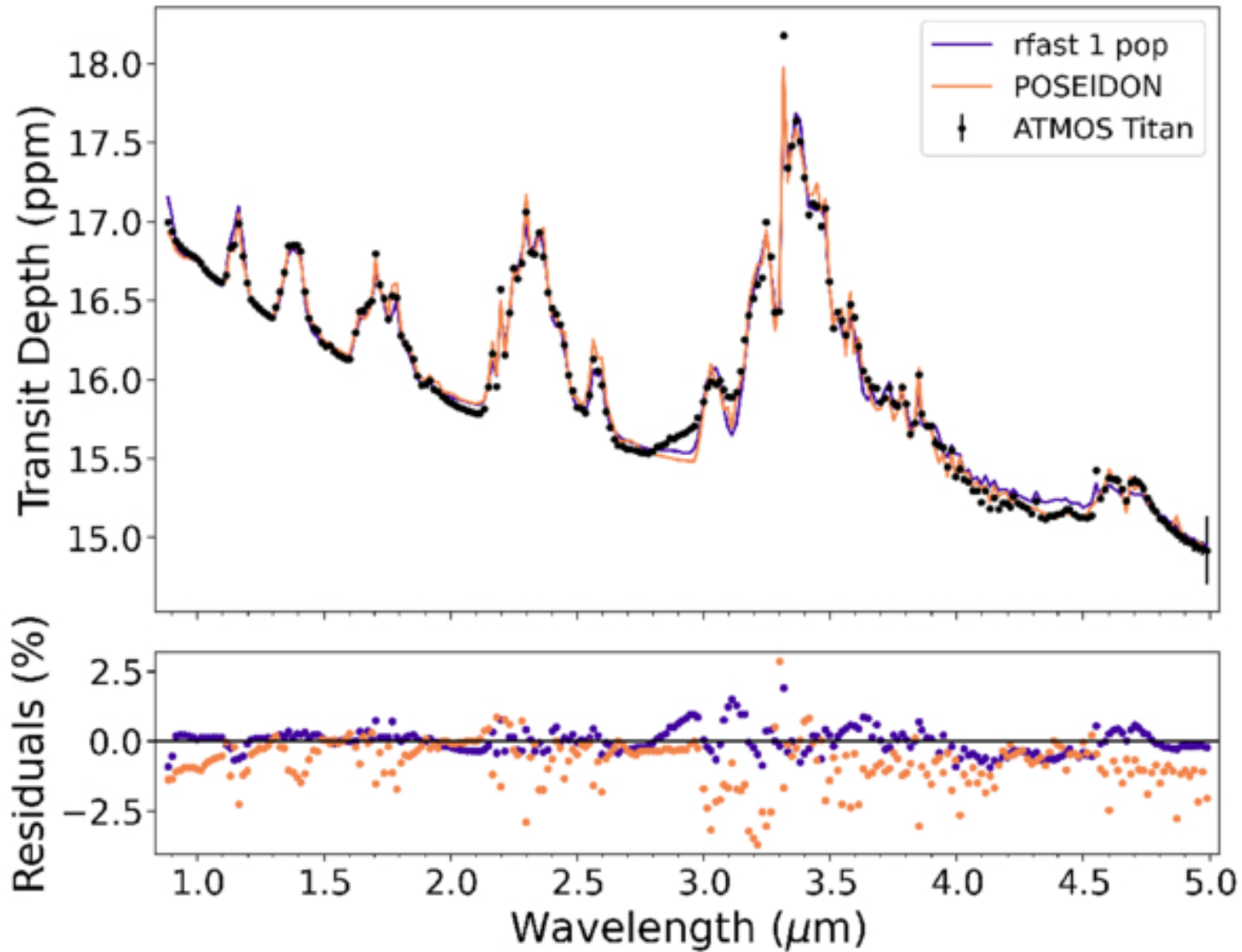
Figure 5. from L. C. Mayorga et al 2026 Astron. J. 172 doi:10.3847/1538-3881/ae7712 https://dx.doi.org/10.3847/1538-3881/ae7712 © 2026. The Author(s). Published by the American Astronomical Society.
