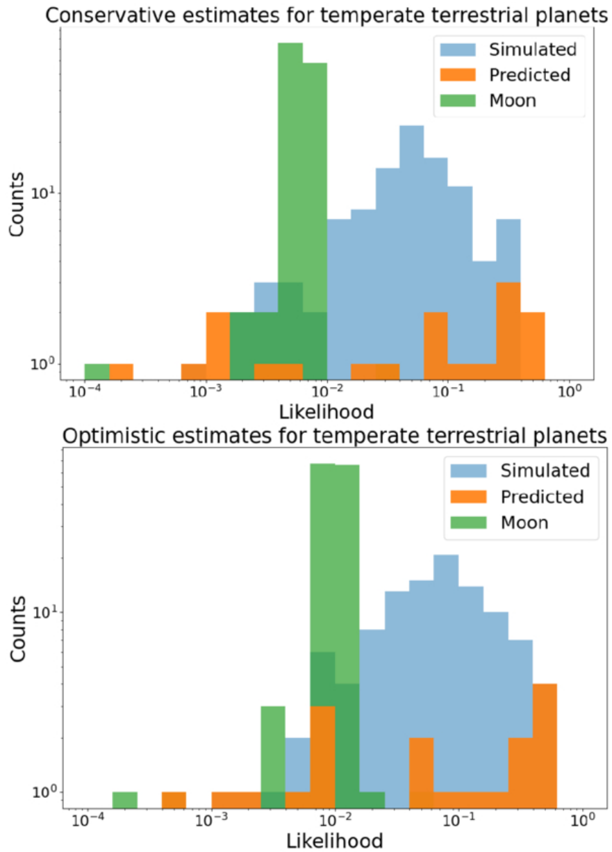
Figure 2. from Jamie Dietrich et al 2026 Astron. J. 172 doi:10.3847/1538-3881/ae76d3 https://dx.doi.org/10.3847/1538-3881/ae76d3 © 2026. The Author(s). Published by the American Astronomical Society.
