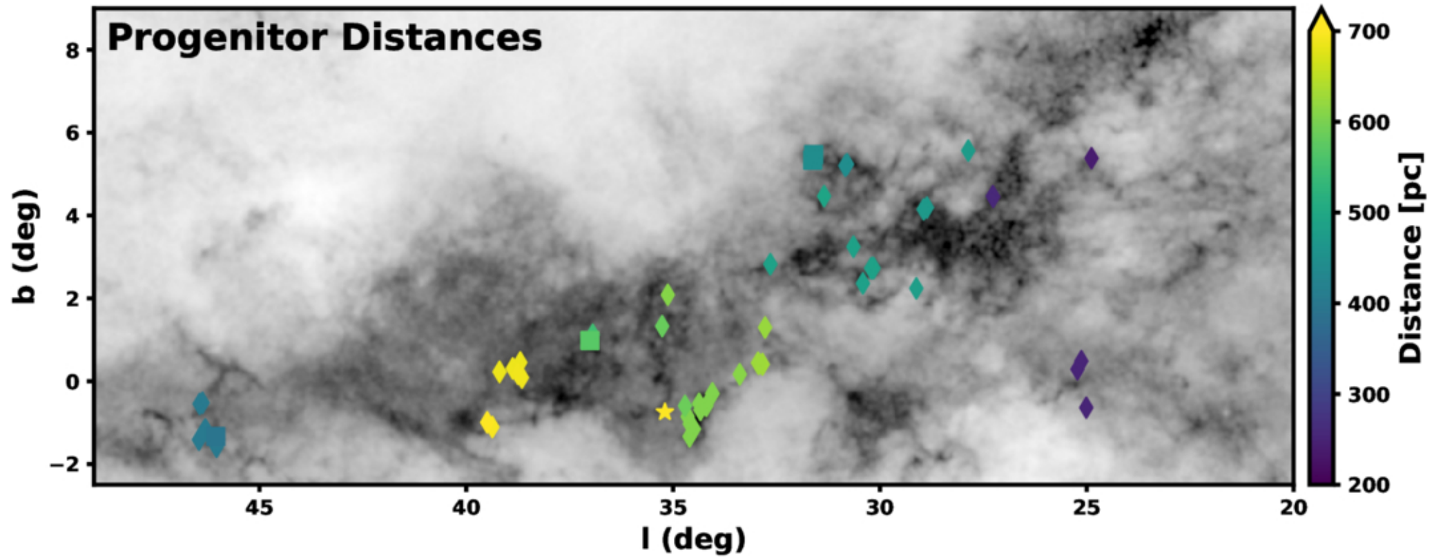
Figure 9. from T. A. Rector et al 2026 Astron. J. 172 doi:10.3847/1538-3881/ae76cb https://dx.doi.org/10.3847/1538-3881/ae76cb © 2026. The Author(s). Published by the American Astronomical Society.
