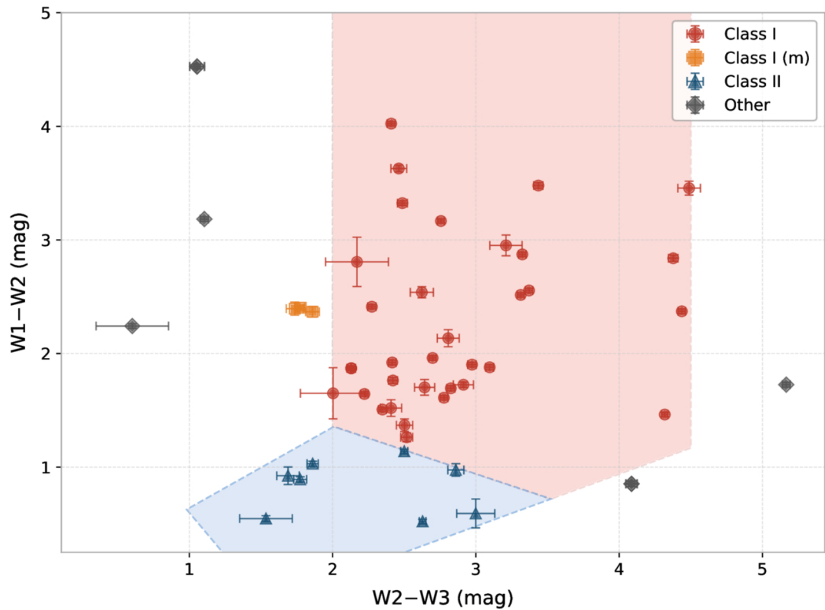
Figure 8. from T. A. Rector et al 2026 Astron. J. 172 doi:10.3847/1538-3881/ae76cb https://dx.doi.org/10.3847/1538-3881/ae76cb © 2026. The Author(s). Published by the American Astronomical Society.
