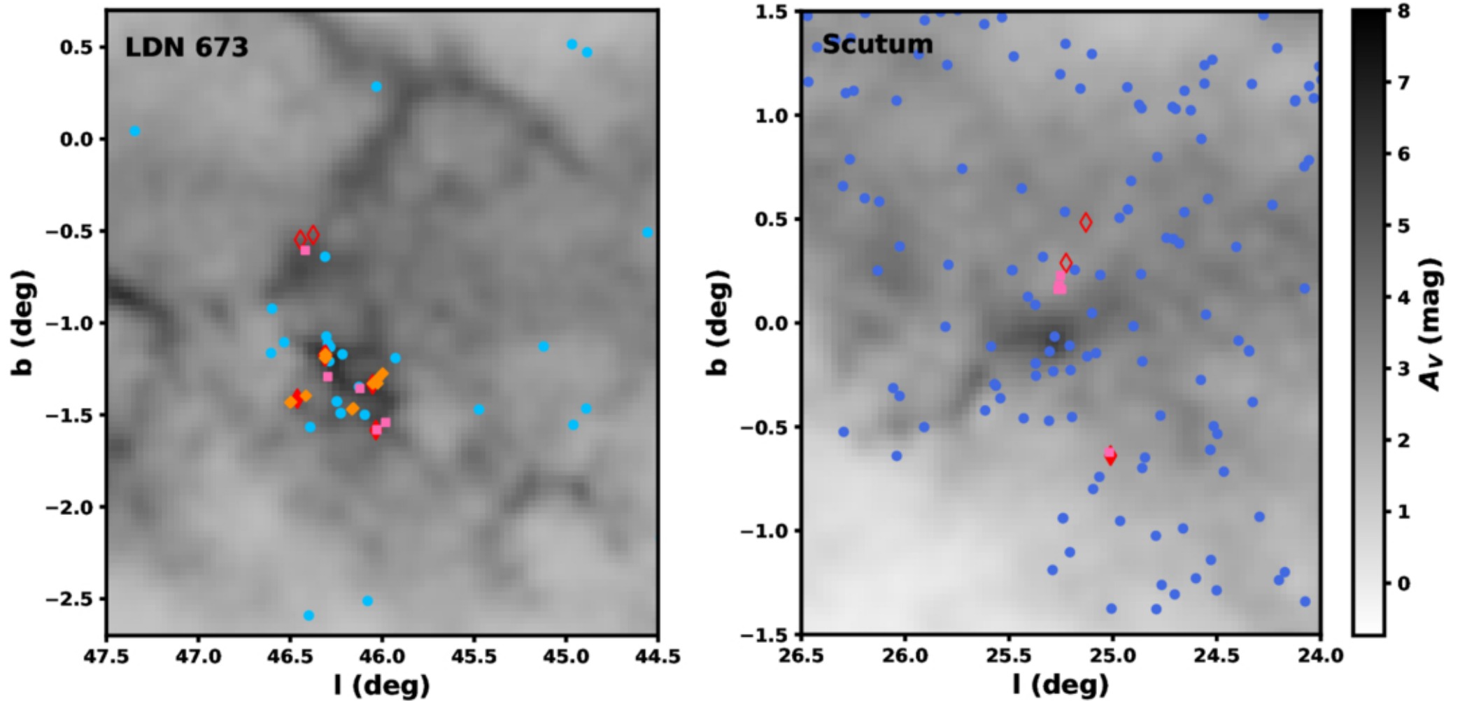
Figure 7. from T. A. Rector et al 2026 Astron. J. 172 doi:10.3847/1538-3881/ae76cb https://dx.doi.org/10.3847/1538-3881/ae76cb © 2026. The Author(s). Published by the American Astronomical Society.
