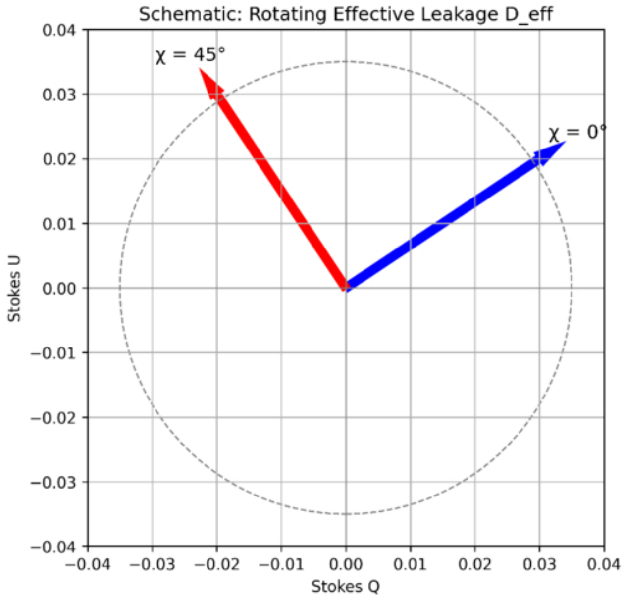
Figure 1. from Dipanjan Mitra 2026 Astron. J. 172 doi:10.3847/1538-3881/ae75ea https://dx.doi.org/10.3847/1538-3881/ae75ea © 2026. The Author(s). Published by the American Astronomical Society.
