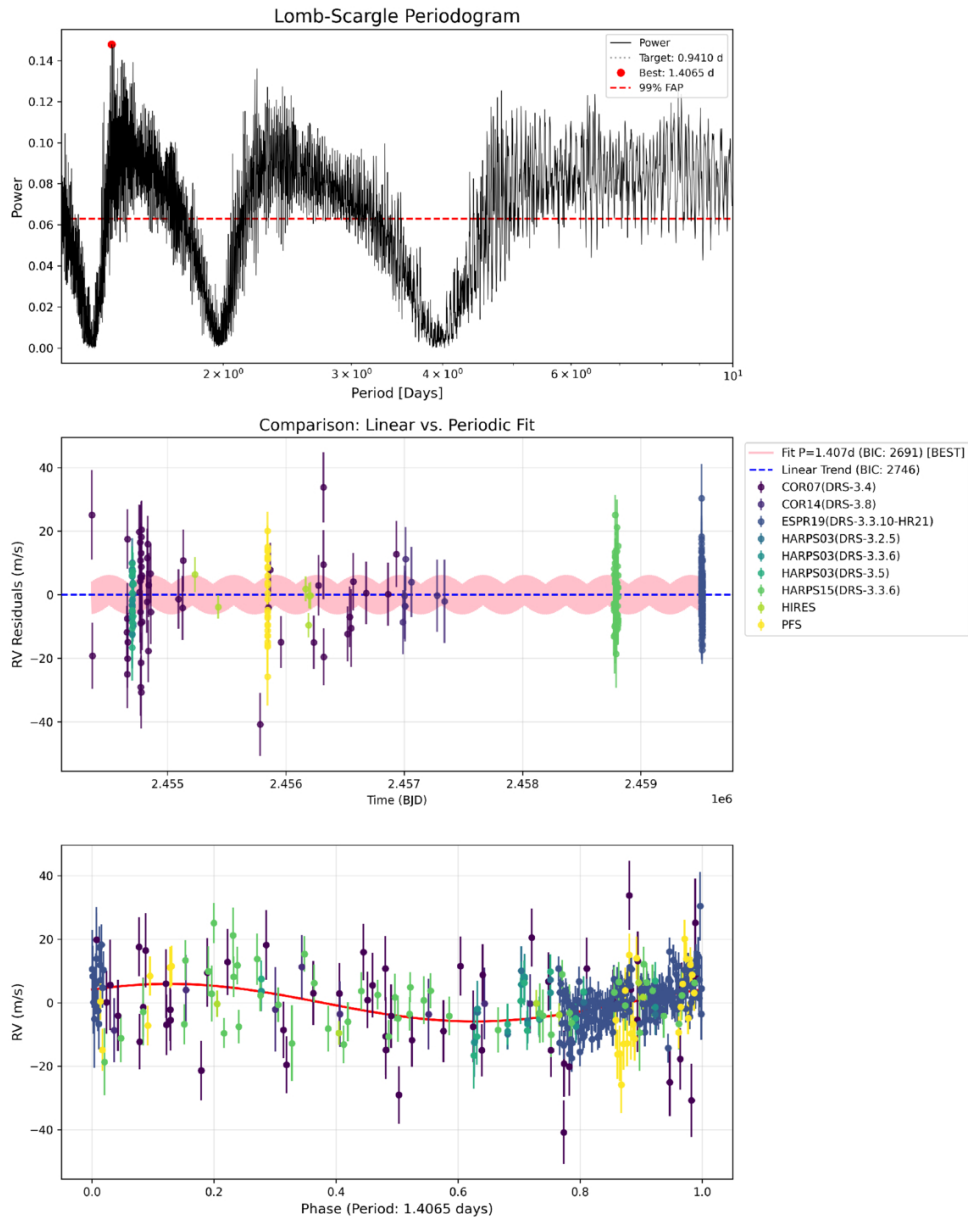
Figure 7. from Avinash S. Nedyedath et al 2026 Astron. J. 172 doi:10.3847/1538-3881/ae75e8 https://dx.doi.org/10.3847/1538-3881/ae75e8 © 2026. The Author(s). Published by the American Astronomical Society.
