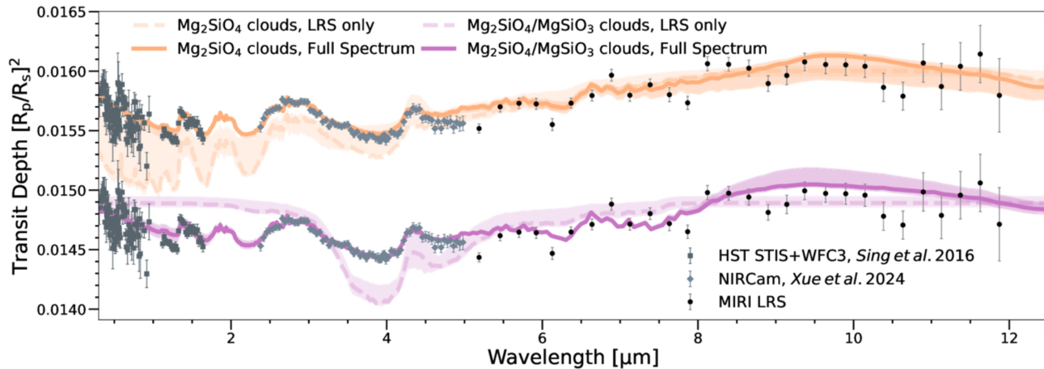
Figure 9. from Katy L. Chubb et al 2026 Astron. J. 172 doi:10.3847/1538-3881/ae75de https://dx.doi.org/10.3847/1538-3881/ae75de © 2026. The Author(s). Published by the American Astronomical Society.
