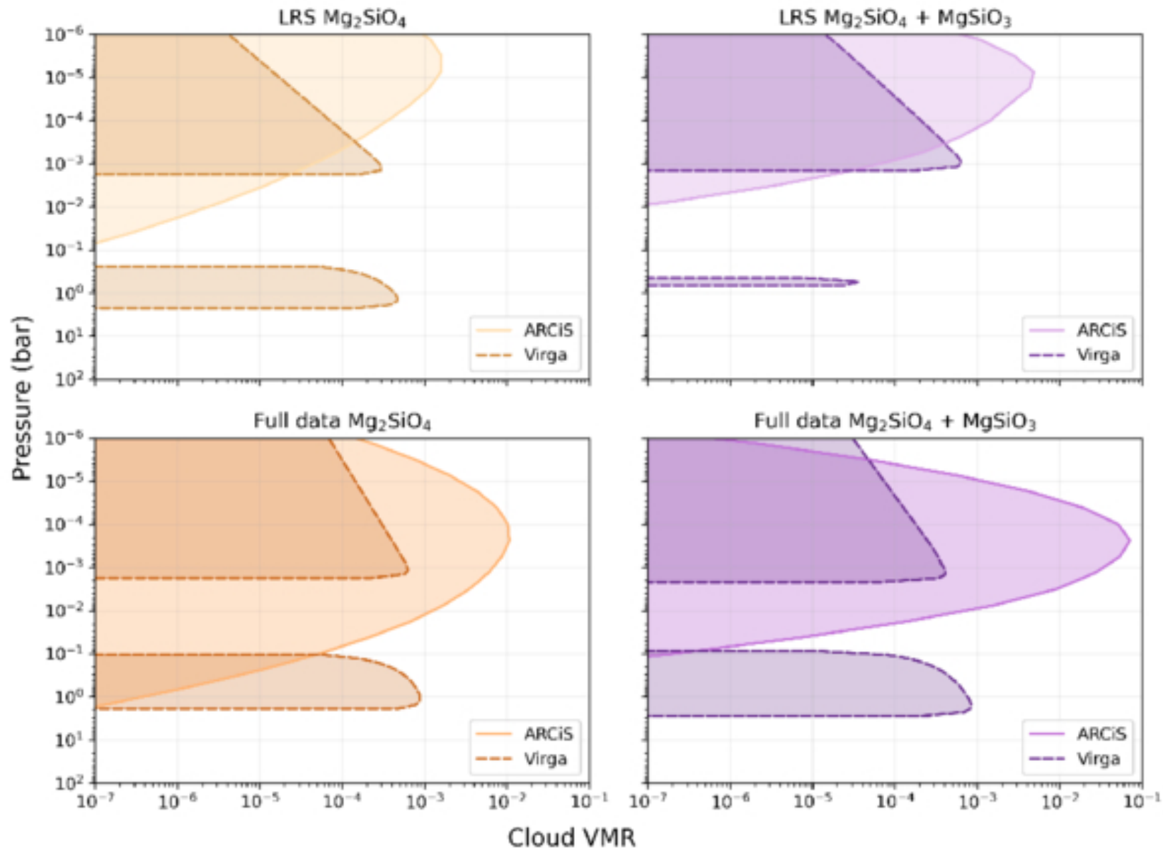
Figure 8. from Katy L. Chubb et al 2026 Astron. J. 172 doi:10.3847/1538-3881/ae75de https://dx.doi.org/10.3847/1538-3881/ae75de © 2026. The Author(s). Published by the American Astronomical Society.
