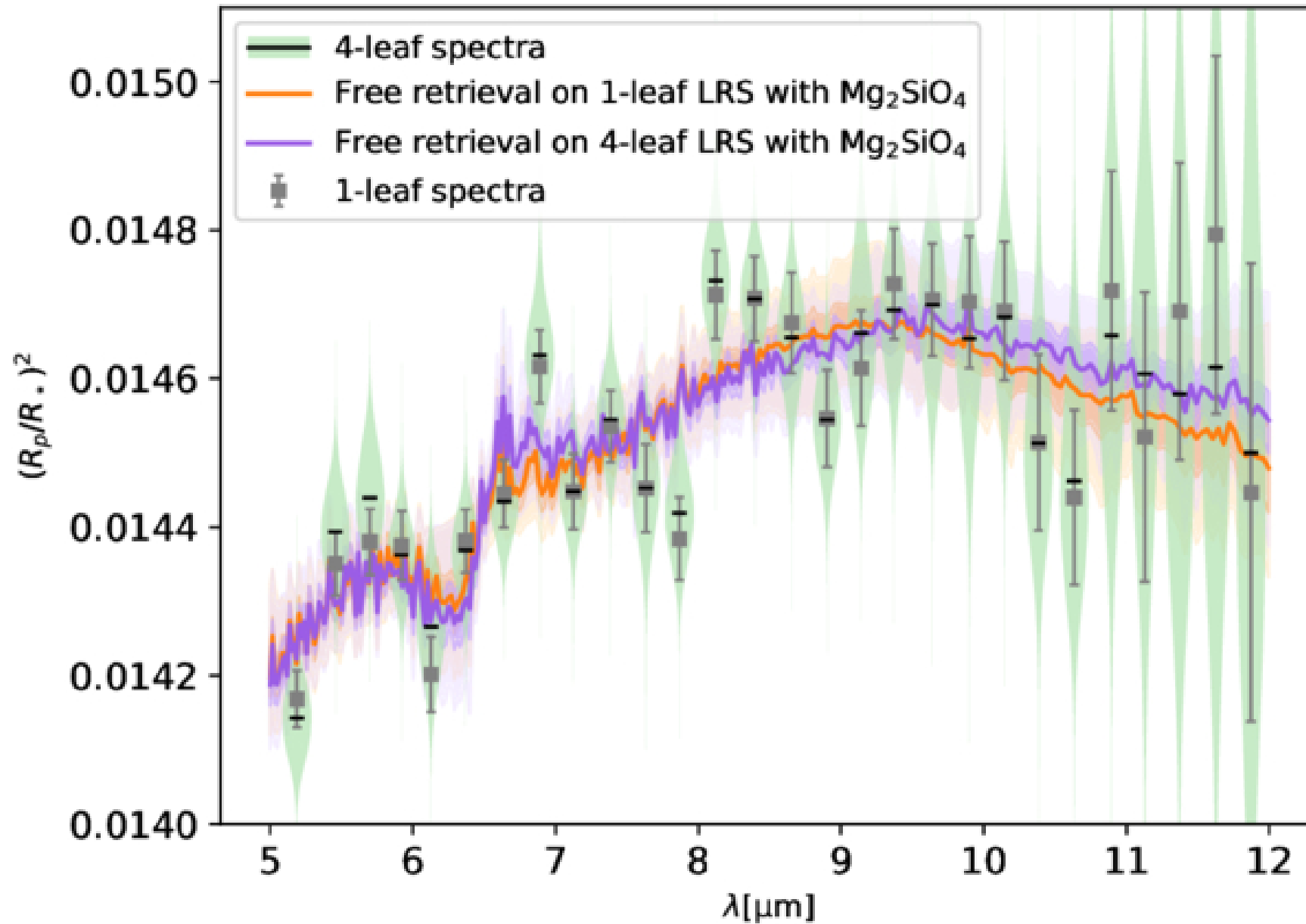
Figure 10. from Katy L. Chubb et al 2026 Astron. J. 172 doi:10.3847/1538-3881/ae75de https://dx.doi.org/10.3847/1538-3881/ae75de © 2026. The Author(s). Published by the American Astronomical Society.
