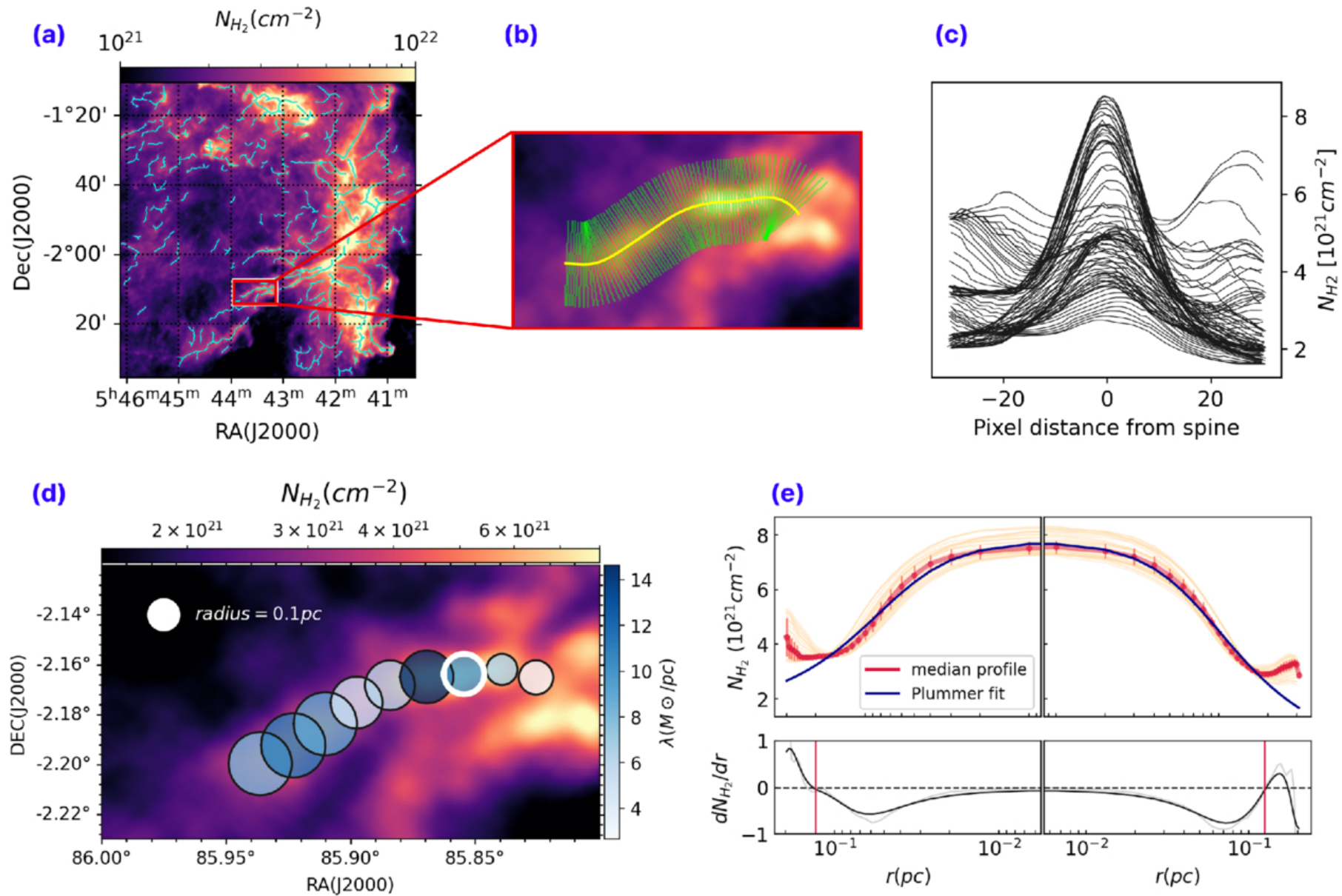
Figure 7. from Shivam Kumaran et al 2026 Astron. J. 172 doi:10.3847/1538-3881/ae75db https://dx.doi.org/10.3847/1538-3881/ae75db © 2026. The Author(s). Published by the American Astronomical Society.
