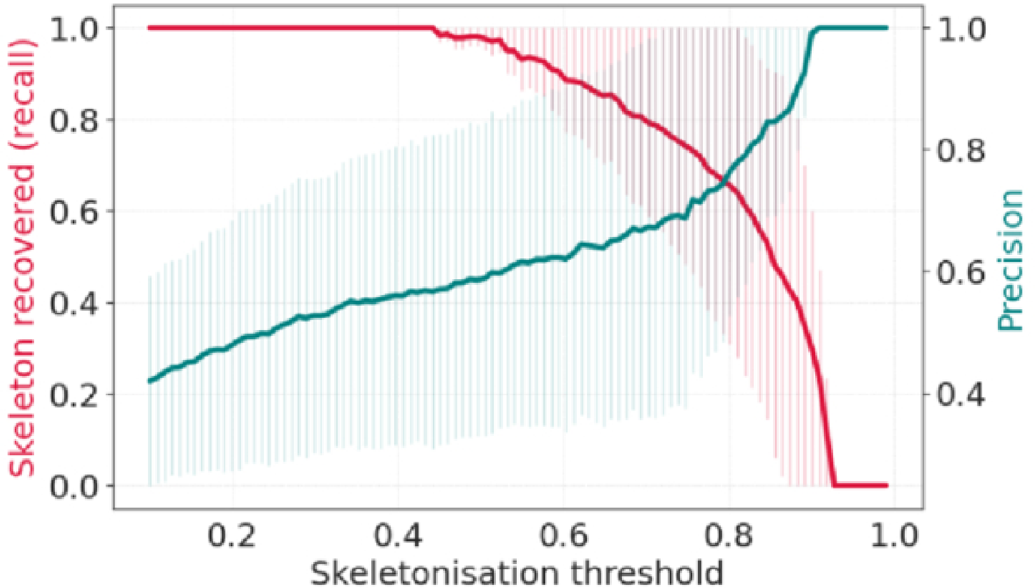
Figure 5. from Shivam Kumaran et al 2026 Astron. J. 172 doi:10.3847/1538-3881/ae75db https://dx.doi.org/10.3847/1538-3881/ae75db © 2026. The Author(s). Published by the American Astronomical Society.
