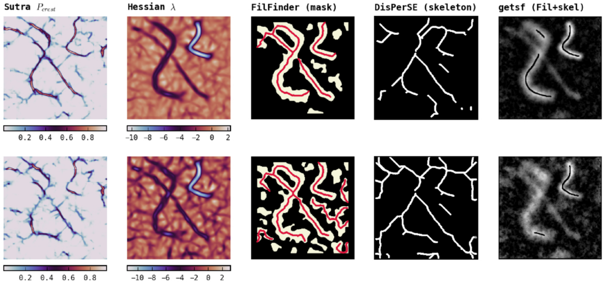
Figure 13. from Shivam Kumaran et al 2026 Astron. J. 172 doi:10.3847/1538-3881/ae75db https://dx.doi.org/10.3847/1538-3881/ae75db © 2026. The Author(s). Published by the American Astronomical Society.
