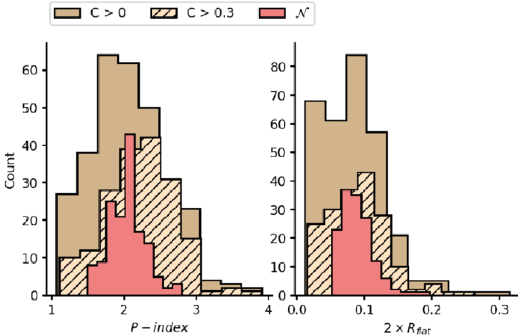
Figure 10. from Shivam Kumaran et al 2026 Astron. J. 172 doi:10.3847/1538-3881/ae75db https://dx.doi.org/10.3847/1538-3881/ae75db © 2026. The Author(s). Published by the American Astronomical Society.
