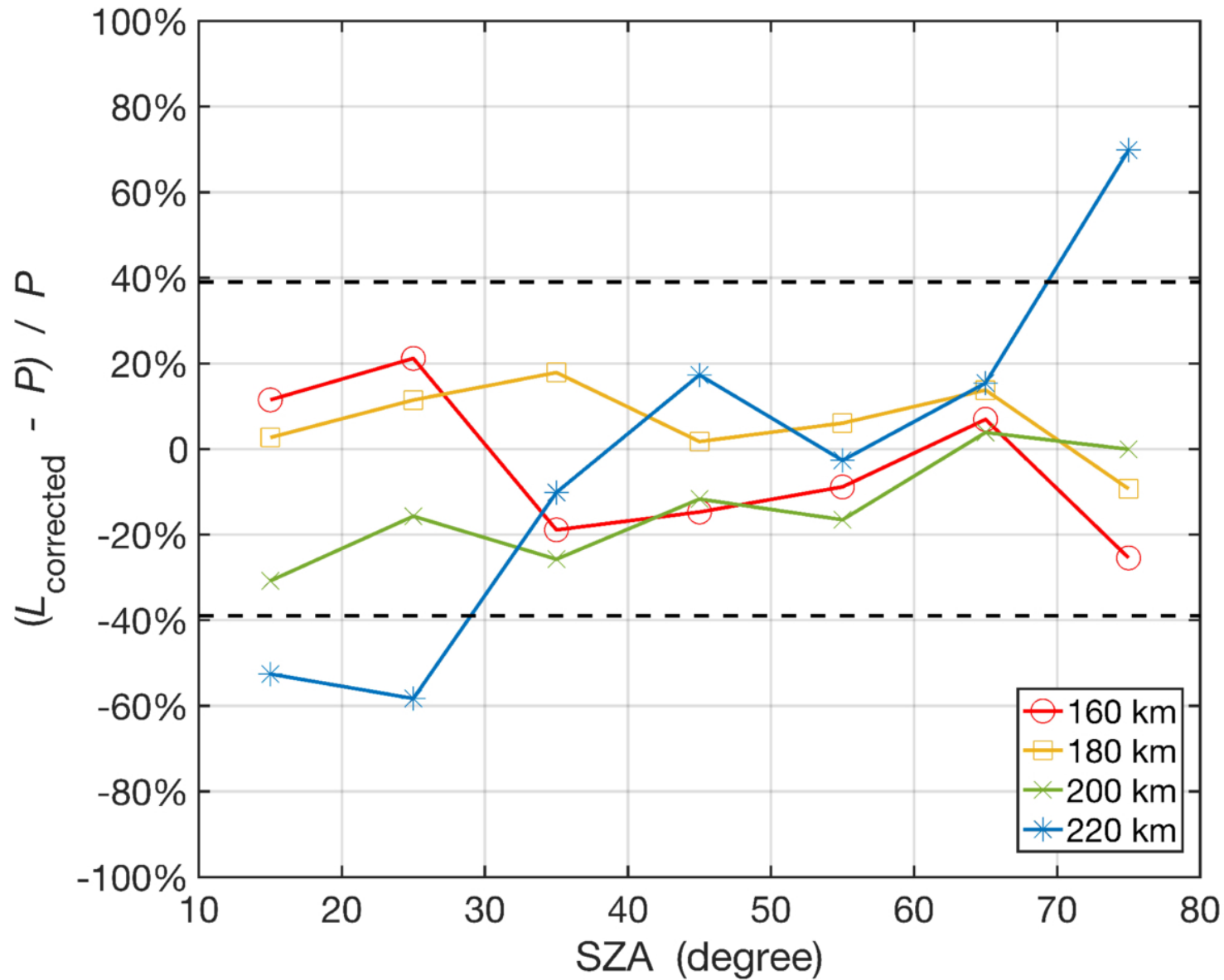
Figure 6. from Wenjun Liang et al 2026 Astron. J. 172 doi:10.3847/1538-3881/ae75af https://dx.doi.org/10.3847/1538-3881/ae75af © 2026. The Author(s). Published by the American Astronomical Society.
