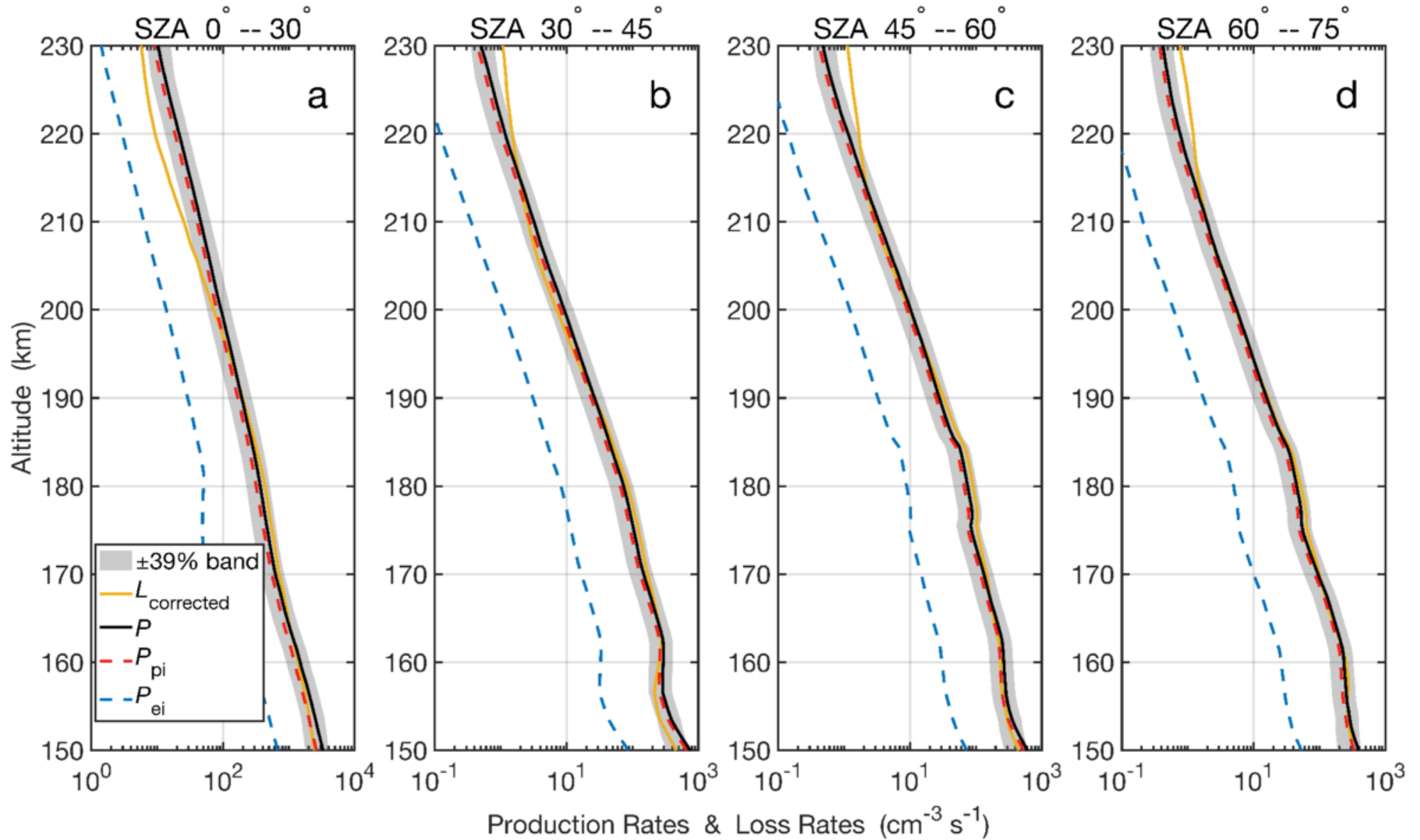
Figure 5. from Wenjun Liang et al 2026 Astron. J. 172 doi:10.3847/1538-3881/ae75af https://dx.doi.org/10.3847/1538-3881/ae75af © 2026. The Author(s). Published by the American Astronomical Society.
