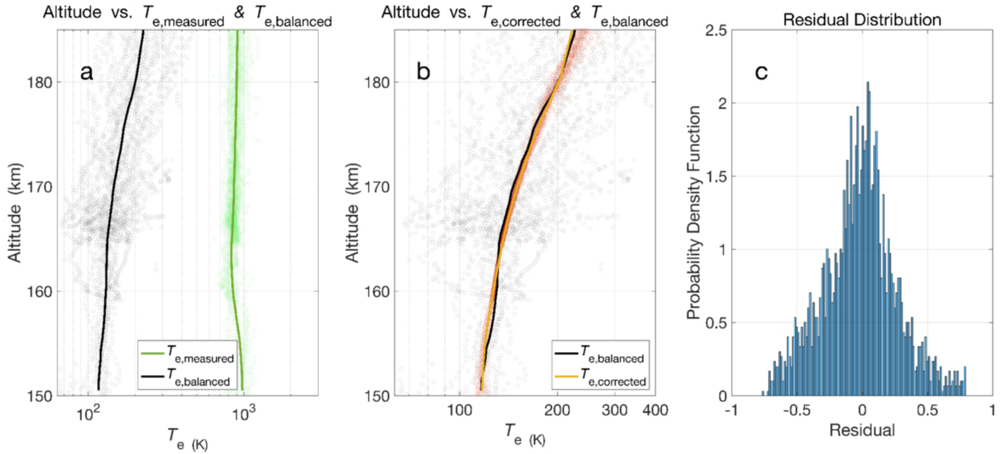
Figure 3. from Wenjun Liang et al 2026 Astron. J. 172 doi:10.3847/1538-3881/ae75af https://dx.doi.org/10.3847/1538-3881/ae75af © 2026. The Author(s). Published by the American Astronomical Society.
