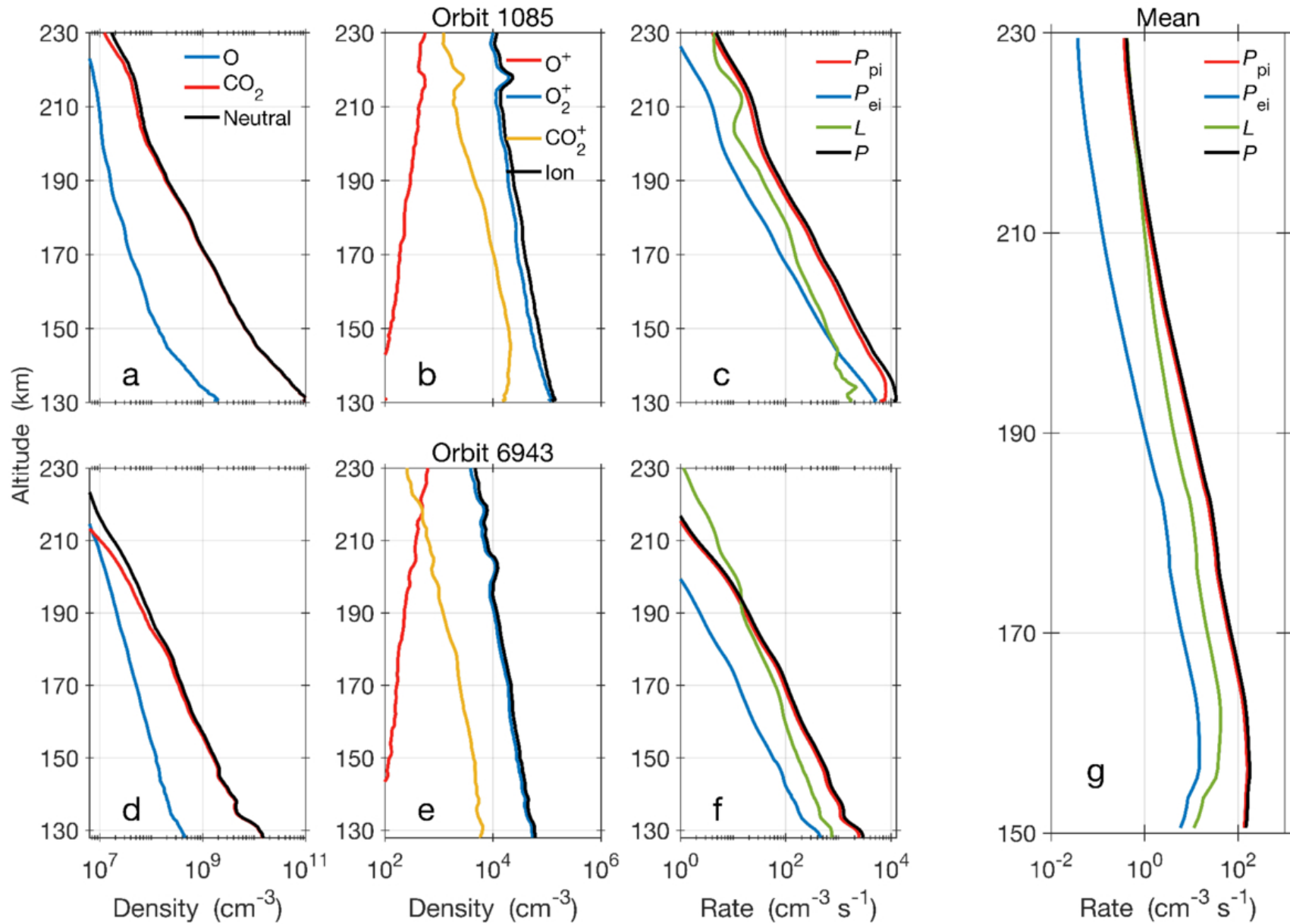
Figure 2. from Wenjun Liang et al 2026 Astron. J. 172 doi:10.3847/1538-3881/ae75af https://dx.doi.org/10.3847/1538-3881/ae75af © 2026. The Author(s). Published by the American Astronomical Society.
