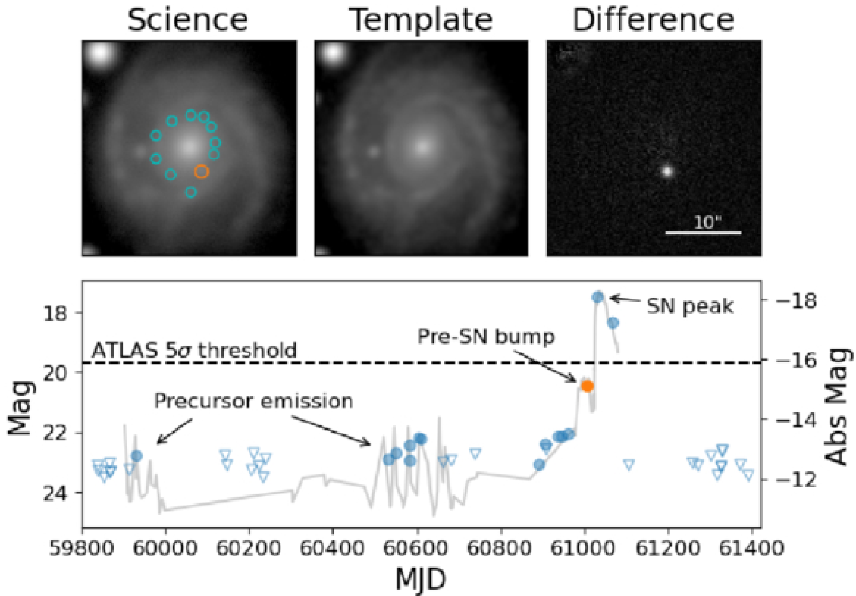
Figure 8. from Tobias Géron et al 2026 Astron. J. 172 doi:10.3847/1538-3881/ae75ad https://dx.doi.org/10.3847/1538-3881/ae75ad © 2026. The Author(s). Published by the American Astronomical Society.
