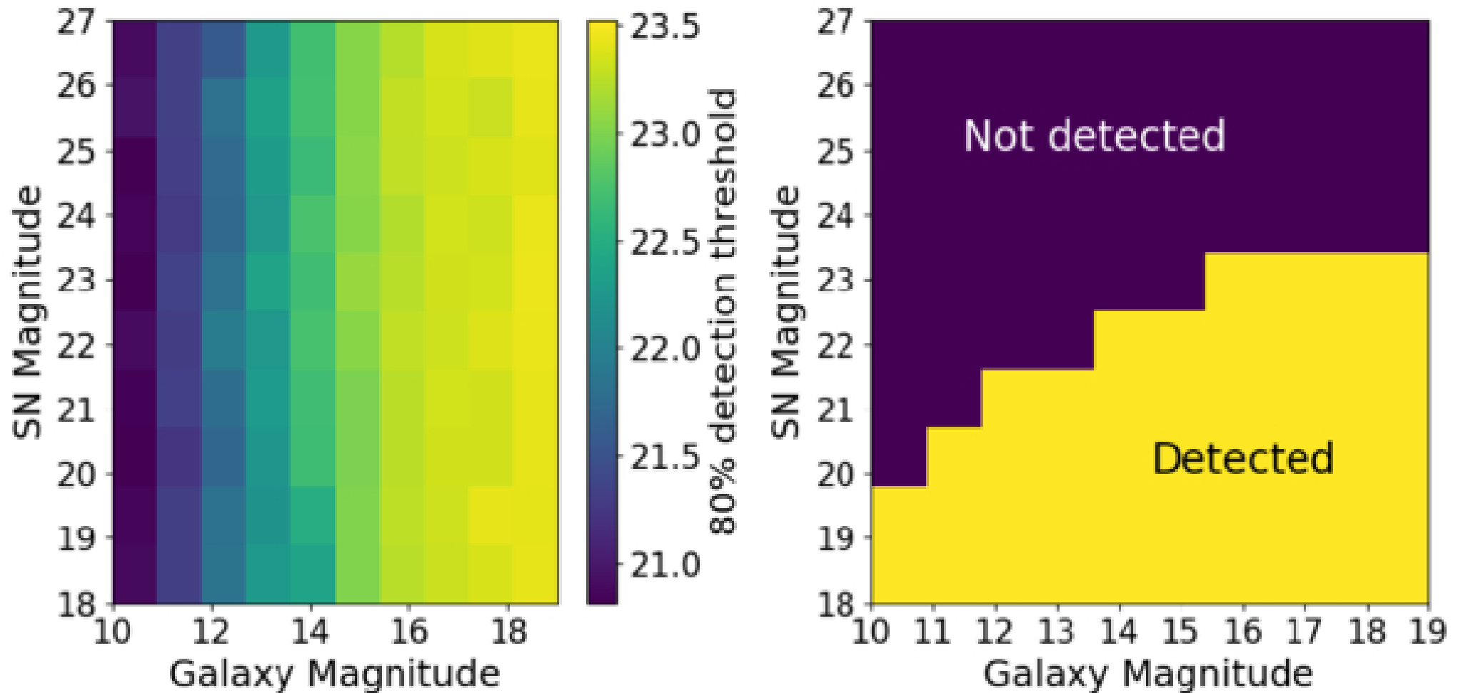
Figure 7. from Tobias Géron et al 2026 Astron. J. 172 doi:10.3847/1538-3881/ae75ad https://dx.doi.org/10.3847/1538-3881/ae75ad © 2026. The Author(s). Published by the American Astronomical Society.
