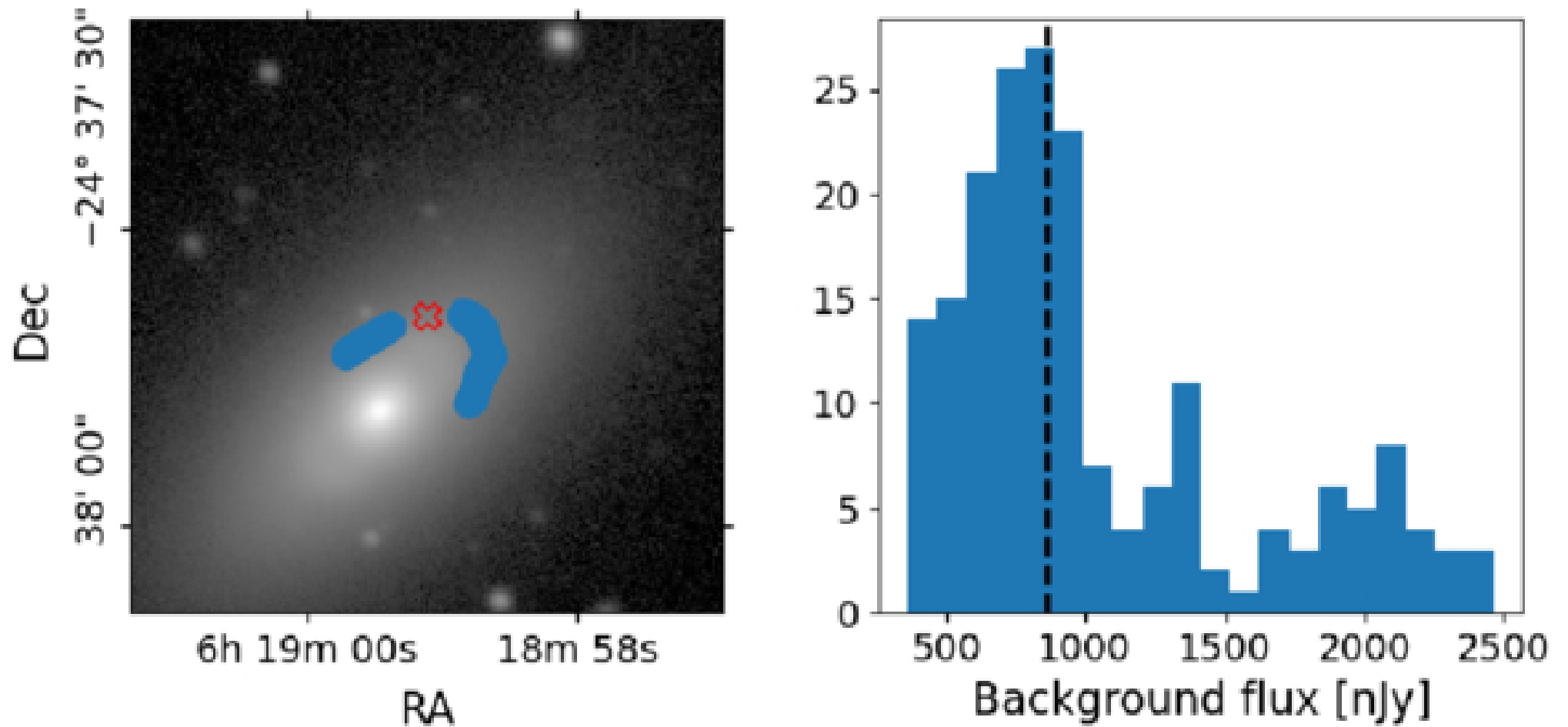
Figure 5. from Tobias Géron et al 2026 Astron. J. 172 doi:10.3847/1538-3881/ae75ad https://dx.doi.org/10.3847/1538-3881/ae75ad © 2026. The Author(s). Published by the American Astronomical Society.
