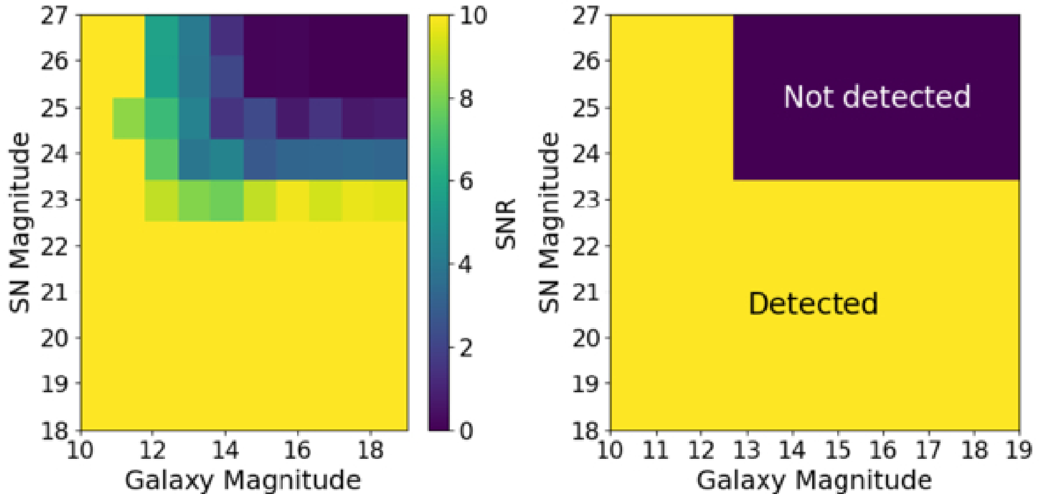
Figure 2. from Tobias Géron et al 2026 Astron. J. 172 doi:10.3847/1538-3881/ae75ad https://dx.doi.org/10.3847/1538-3881/ae75ad © 2026. The Author(s). Published by the American Astronomical Society.
