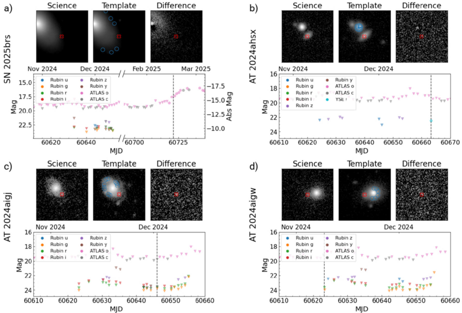
Figure 10. from Tobias Géron et al 2026 Astron. J. 172 doi:10.3847/1538-3881/ae75ad https://dx.doi.org/10.3847/1538-3881/ae75ad © 2026. The Author(s). Published by the American Astronomical Society.
