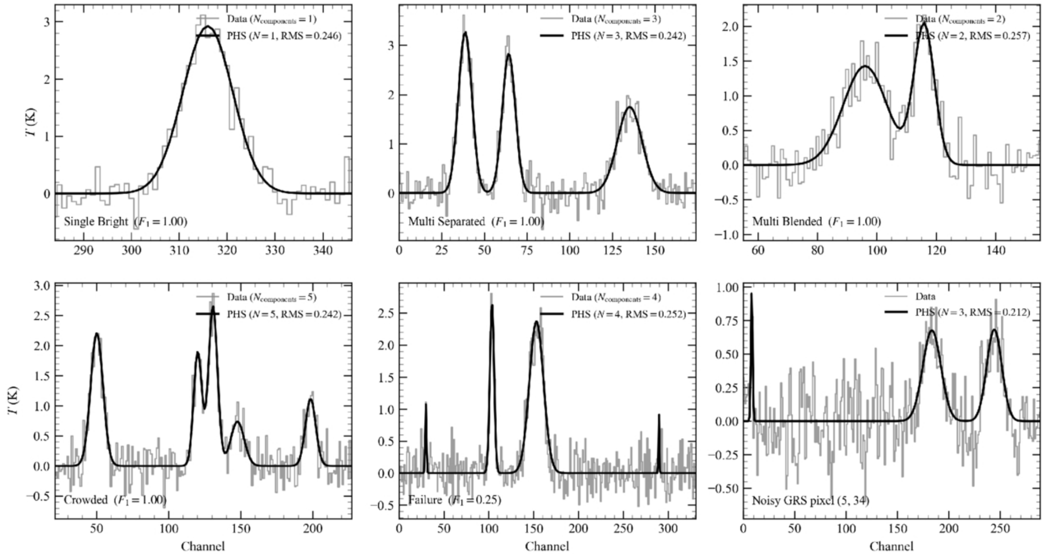
Figure 4. from Carlos Vera-Ciro 2026 Astron. J. 172 doi:10.3847/1538-3881/ae7435 https://dx.doi.org/10.3847/1538-3881/ae7435 © 2026. The Author(s). Published by the American Astronomical Society.
