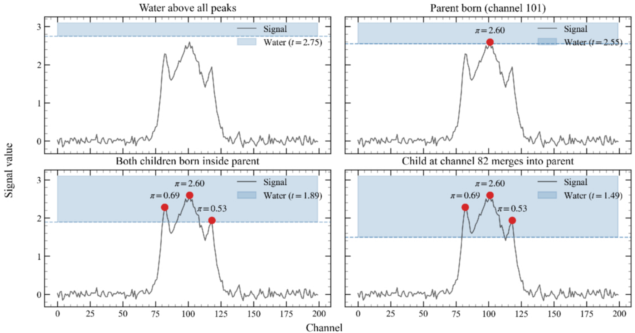
Figure 1. from Carlos Vera-Ciro 2026 Astron. J. 172 doi:10.3847/1538-3881/ae7435 https://dx.doi.org/10.3847/1538-3881/ae7435 © 2026. The Author(s). Published by the American Astronomical Society.
