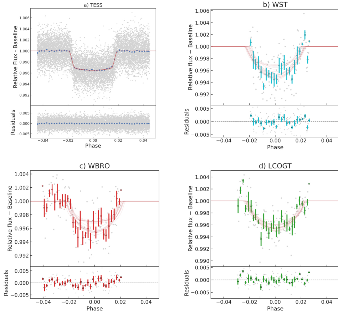
Figure 7. from Md Redyan Ahmed et al 2026 Astron. J. 172 doi:10.3847/1538-3881/ae7370 https://dx.doi.org/10.3847/1538-3881/ae7370 © 2026. The Author(s). Published by the American Astronomical Society.
