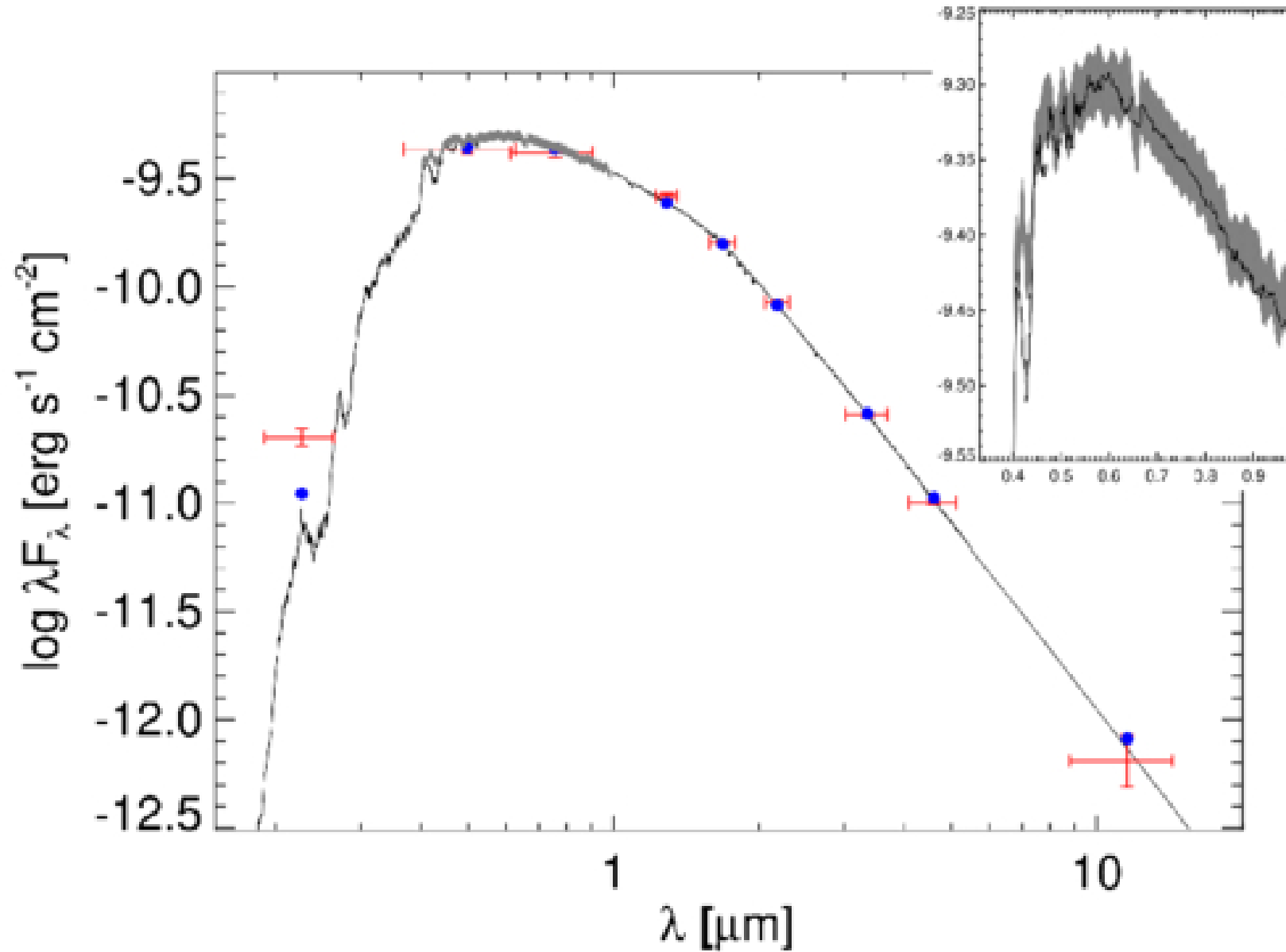
Figure 5. from Md Redyan Ahmed et al 2026 Astron. J. 172 doi:10.3847/1538-3881/ae7370 https://dx.doi.org/10.3847/1538-3881/ae7370 © 2026. The Author(s). Published by the American Astronomical Society.
