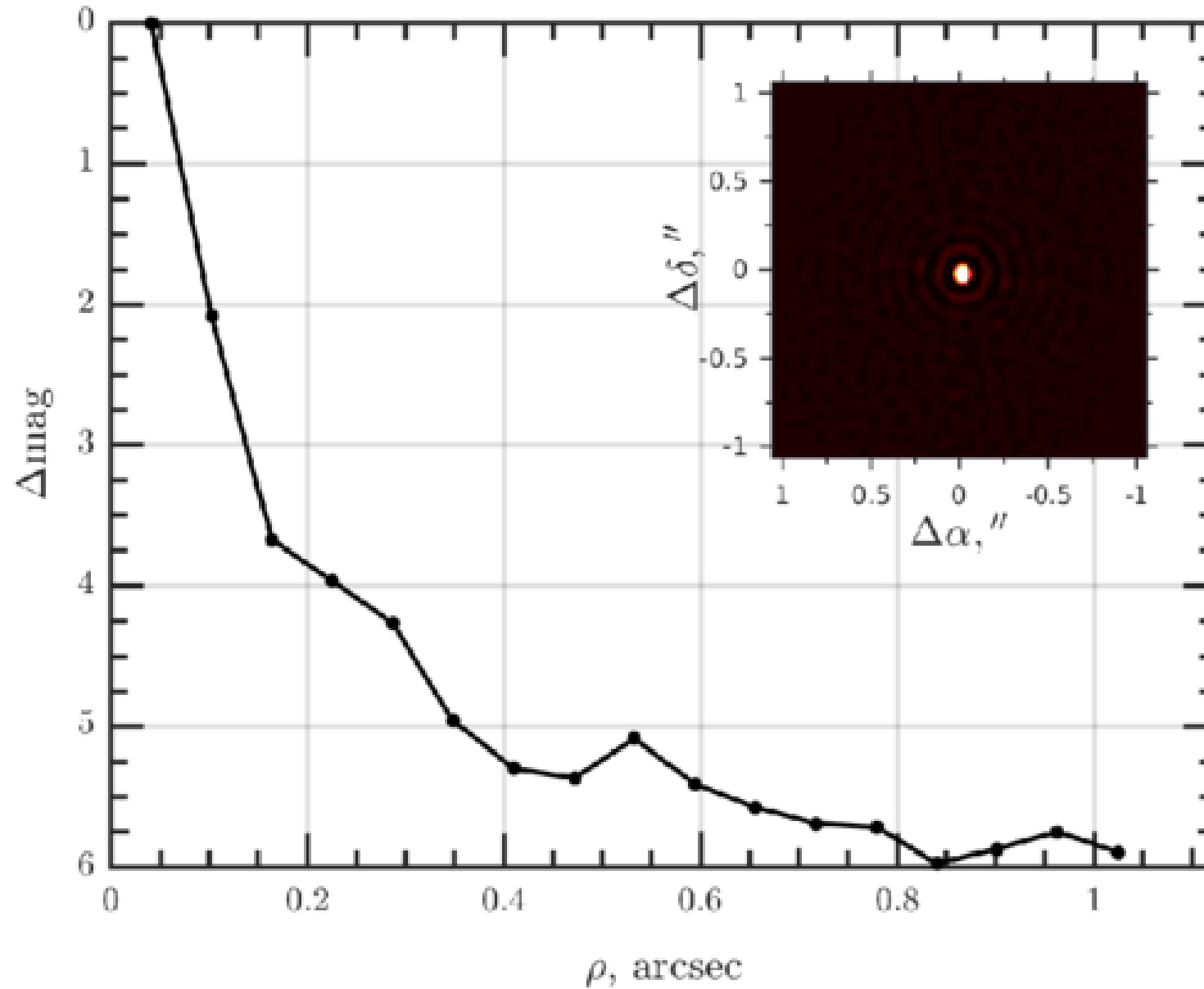
Figure 3. from Md Redyan Ahmed et al 2026 Astron. J. 172 doi:10.3847/1538-3881/ae7370 https://dx.doi.org/10.3847/1538-3881/ae7370 © 2026. The Author(s). Published by the American Astronomical Society.
