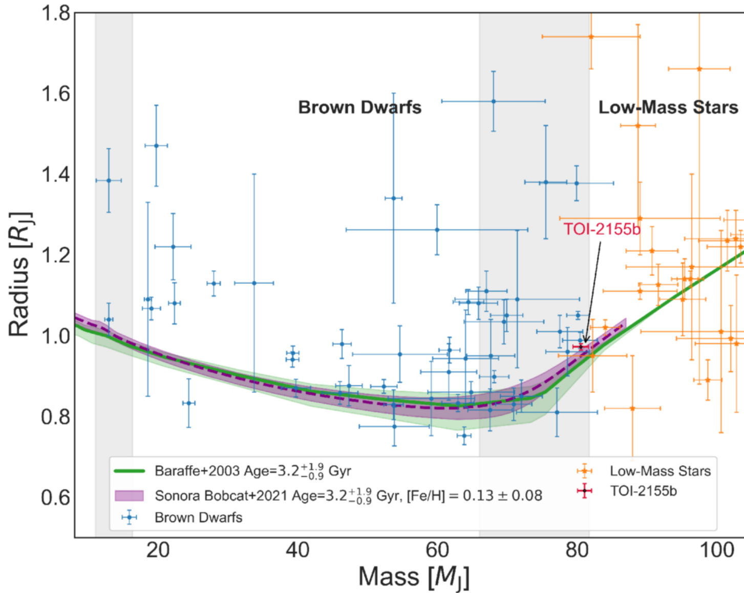
Figure 11. from Md Redyan Ahmed et al 2026 Astron. J. 172 doi:10.3847/1538-3881/ae7370 https://dx.doi.org/10.3847/1538-3881/ae7370 © 2026. The Author(s). Published by the American Astronomical Society.
