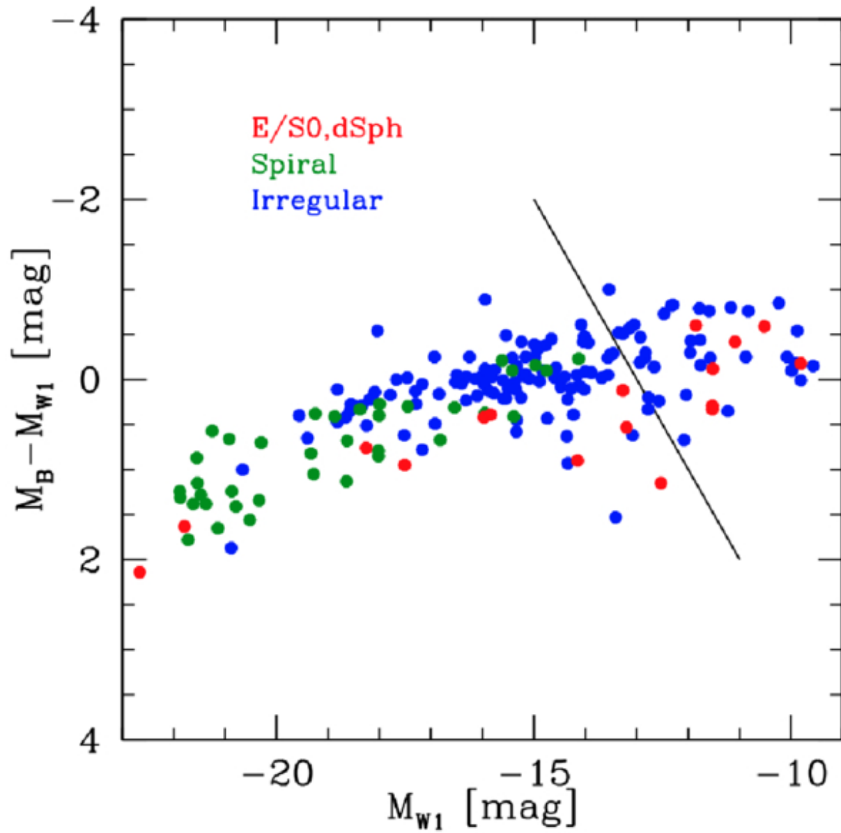
Figure 5. from R. Brent Tully et al 2026 Astron. J. 172 doi:10.3847/1538-3881/ae7330 https://dx.doi.org/10.3847/1538-3881/ae7330 © 2026. The Author(s). Published by the American Astronomical Society.
