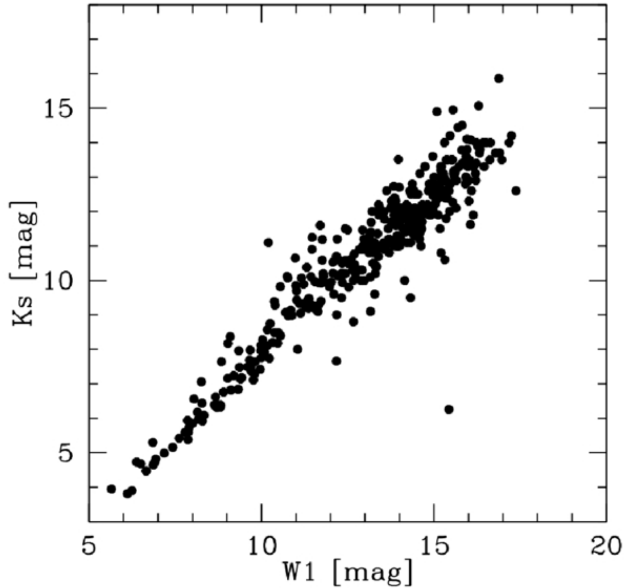
Figure 3. from R. Brent Tully et al 2026 Astron. J. 172 doi:10.3847/1538-3881/ae7330 https://dx.doi.org/10.3847/1538-3881/ae7330 © 2026. The Author(s). Published by the American Astronomical Society.
