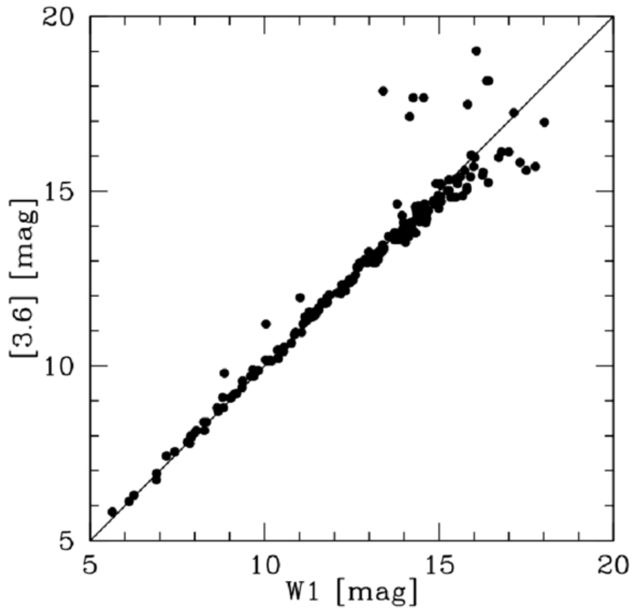
Figure 2. from R. Brent Tully et al 2026 Astron. J. 172 doi:10.3847/1538-3881/ae7330 https://dx.doi.org/10.3847/1538-3881/ae7330 © 2026. The Author(s). Published by the American Astronomical Society.
