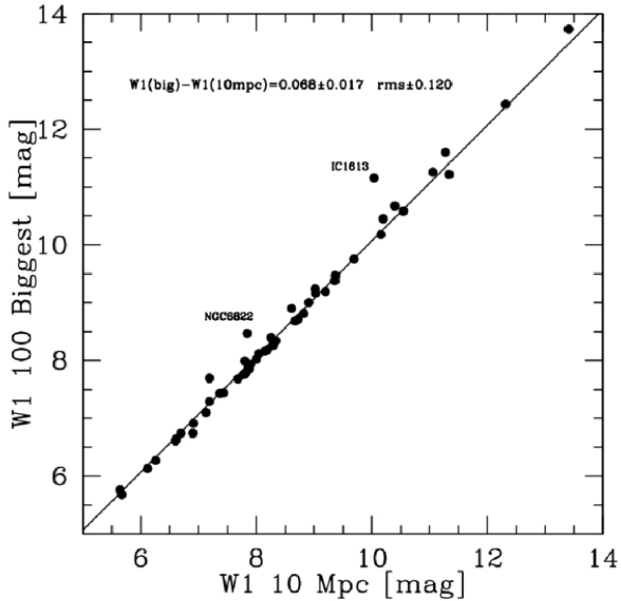
Figure 1. from R. Brent Tully et al 2026 Astron. J. 172 doi:10.3847/1538-3881/ae7330 https://dx.doi.org/10.3847/1538-3881/ae7330 © 2026. The Author(s). Published by the American Astronomical Society.
