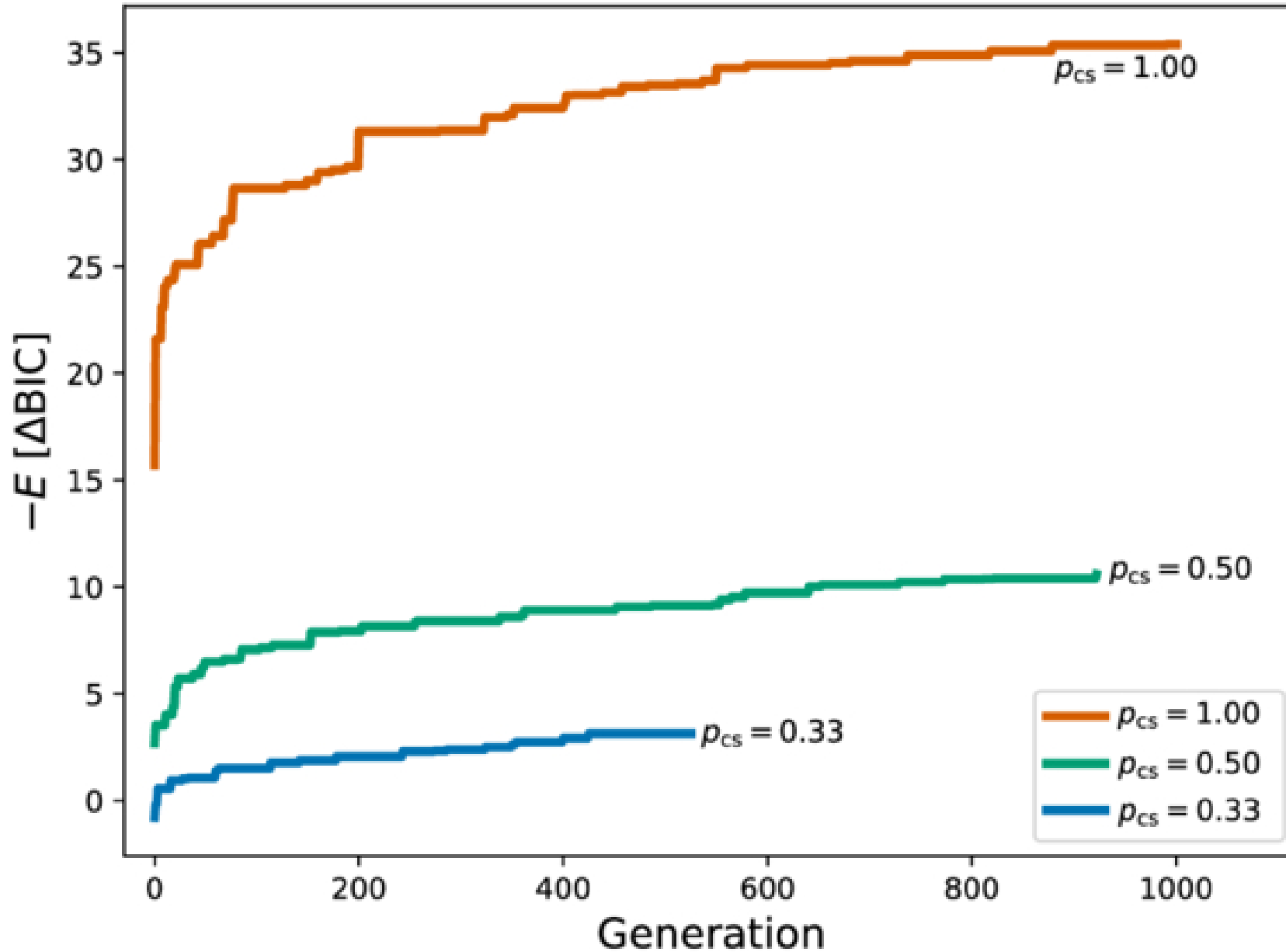
Figure 8. from Jegug lh et al 2026 Astron. J. 172 doi:10.3847/1538-3881/ae71c1 https://dx.doi.org/10.3847/1538-3881/ae71c1 © 2026. The Author(s). Published by the American Astronomical Society.
