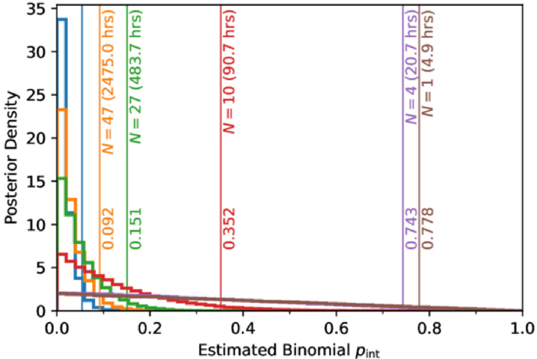
Figure 7. from Jegug lh et al 2026 Astron. J. 172 doi:10.3847/1538-3881/ae71c1 https://dx.doi.org/10.3847/1538-3881/ae71c1 © 2026. The Author(s). Published by the American Astronomical Society.
