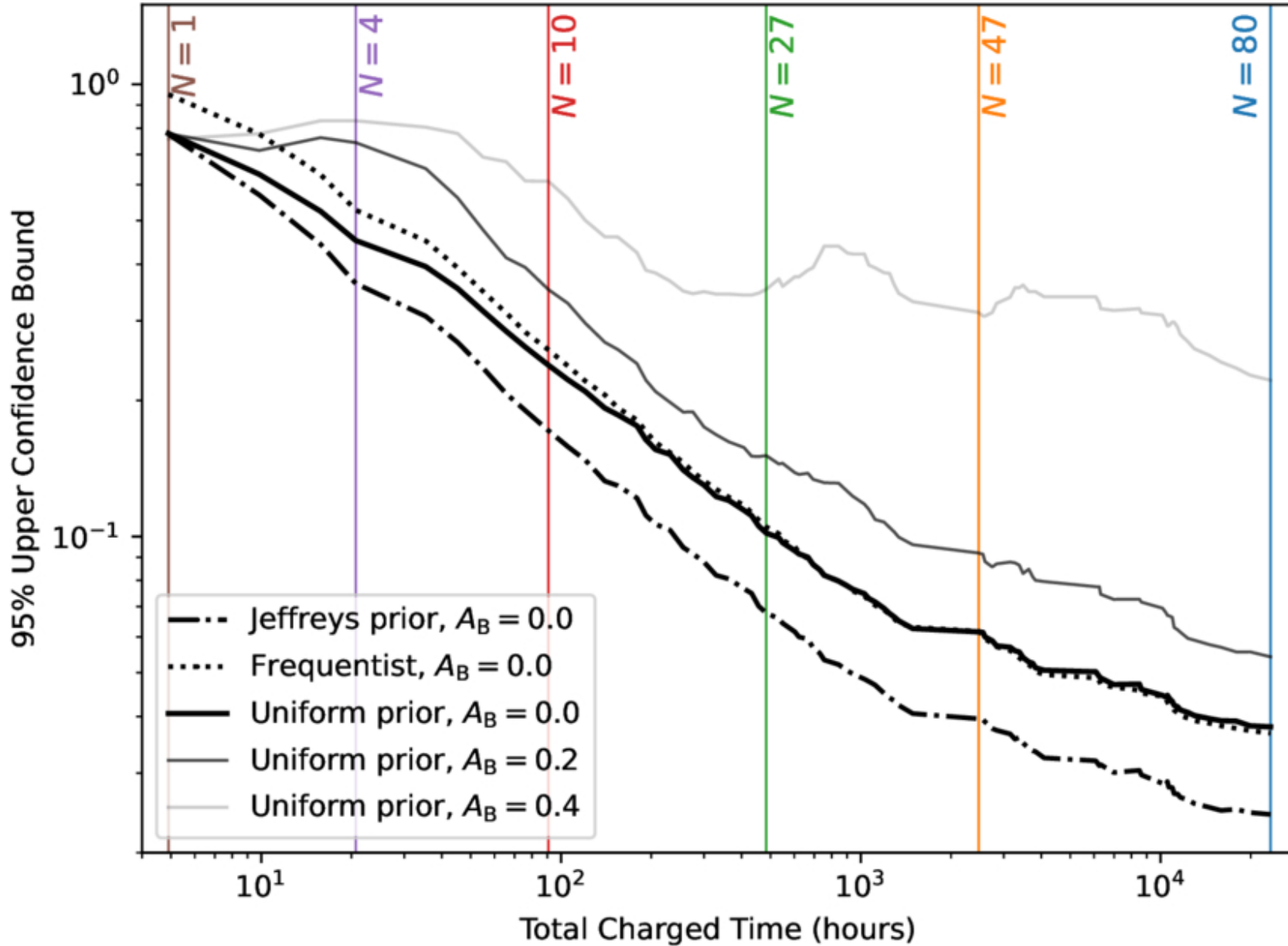
Figure 6. from Jegug lh et al 2026 Astron. J. 172 doi:10.3847/1538-3881/ae71c1 https://dx.doi.org/10.3847/1538-3881/ae71c1 © 2026. The Author(s). Published by the American Astronomical Society.
