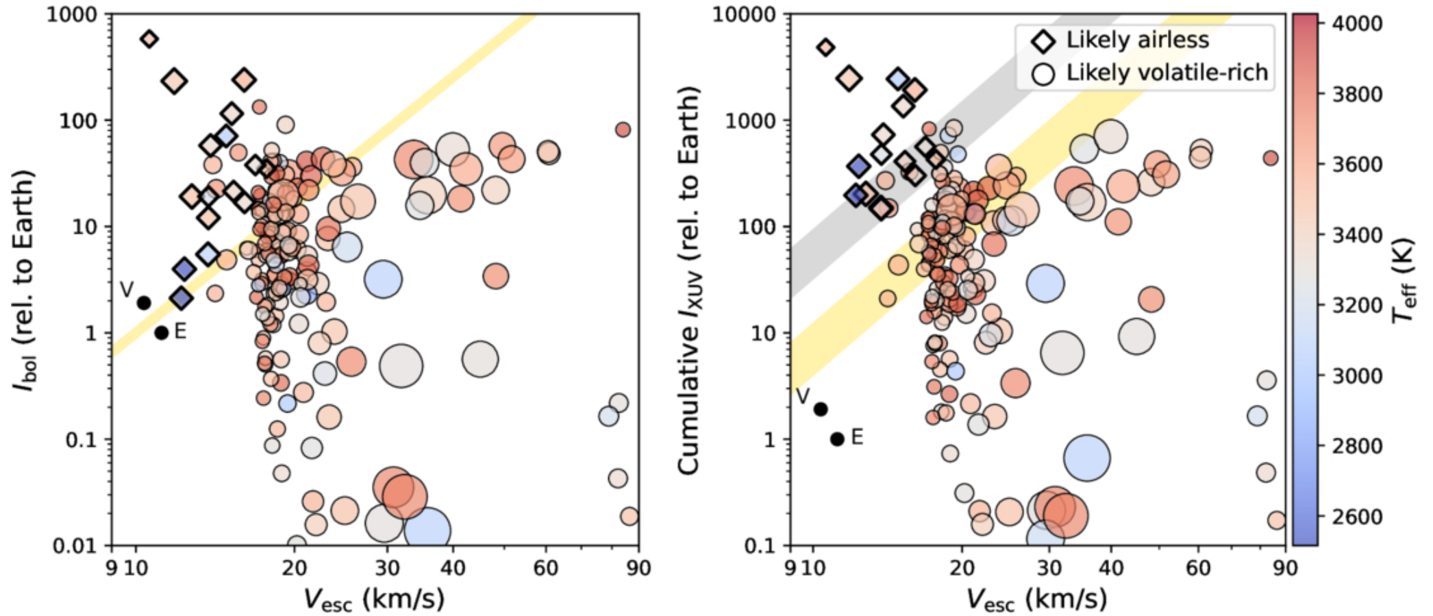
Figure 16. from Jegug Ih et al 2026 Astron. J. 172 doi:10.3847/1538-3881/ae71c1 https://dx.doi.org/10.3847/1538-3881/ae71c1 © 2026. The Author(s). Published by the American Astronomical Society.
