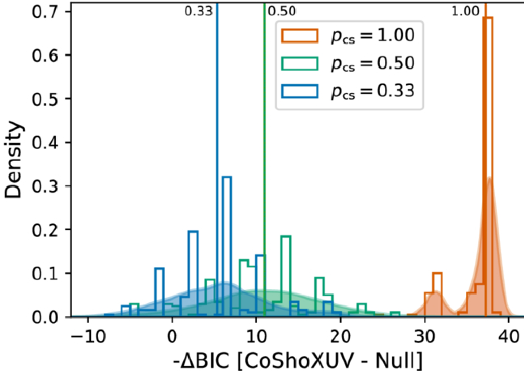
Figure 11. from Jegug lh et al 2026 Astron. J. 172 doi:10.3847/1538-3881/ae71c1 https://dx.doi.org/10.3847/1538-3881/ae71c1 © 2026. The Author(s). Published by the American Astronomical Society.
