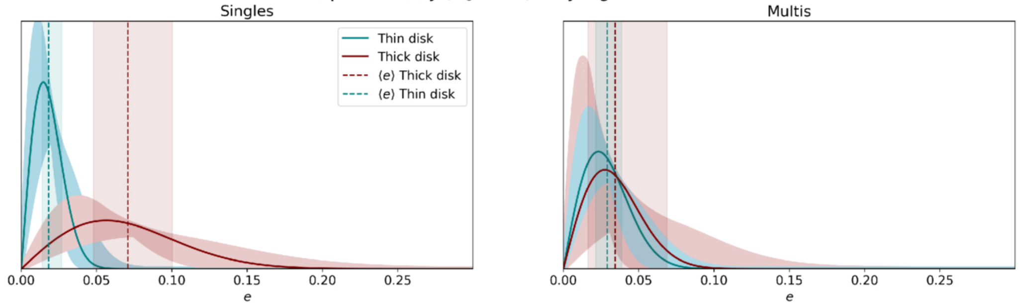
Figure 8. from Sheila Saguear et al 2026 Astron. J. 172 doi:10.3847/1538-3881/ae71bf https://dx.doi.org/10.3847/1538-3881/ae71bf © 2026. The Author(s). Published by the American Astronomical Society.
