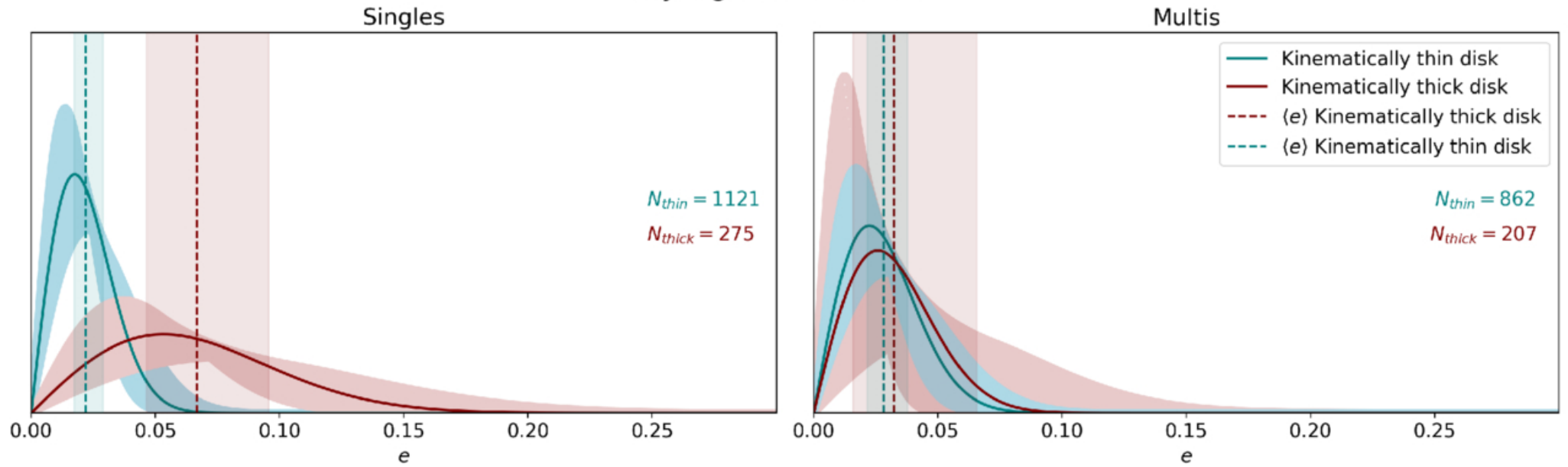
Figure 5. from Sheila Sagar et al 2026 Astron. J. 172 doi:10.3847/1538-3881/ae71bf https://dx.doi.org/10.3847/1538-3881/ae71bf © 2026. The Author(s). Published by the American Astronomical Society.
