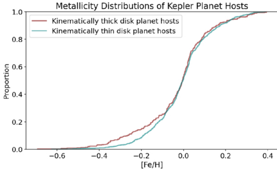
Figure 4. from Sheila Sagar et al 2026 Astron. J. 172 doi:10.3847/1538-3881/ae71bf https://dx.doi.org/10.3847/1538-3881/ae71bf © 2026. The Author(s). Published by the American Astronomical Society.
