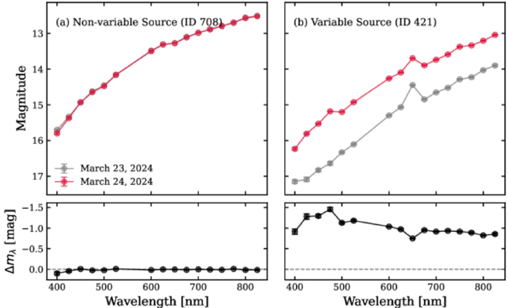
Figure 6. from Mi-Ryang Kim et al 2026 Astron. J. 172 doi:10.3847/1538-3881/ae707f https://dx.doi.org/10.3847/1538-3881/ae707f © 2026. The Author(s). Published by the American Astronomical Society.
