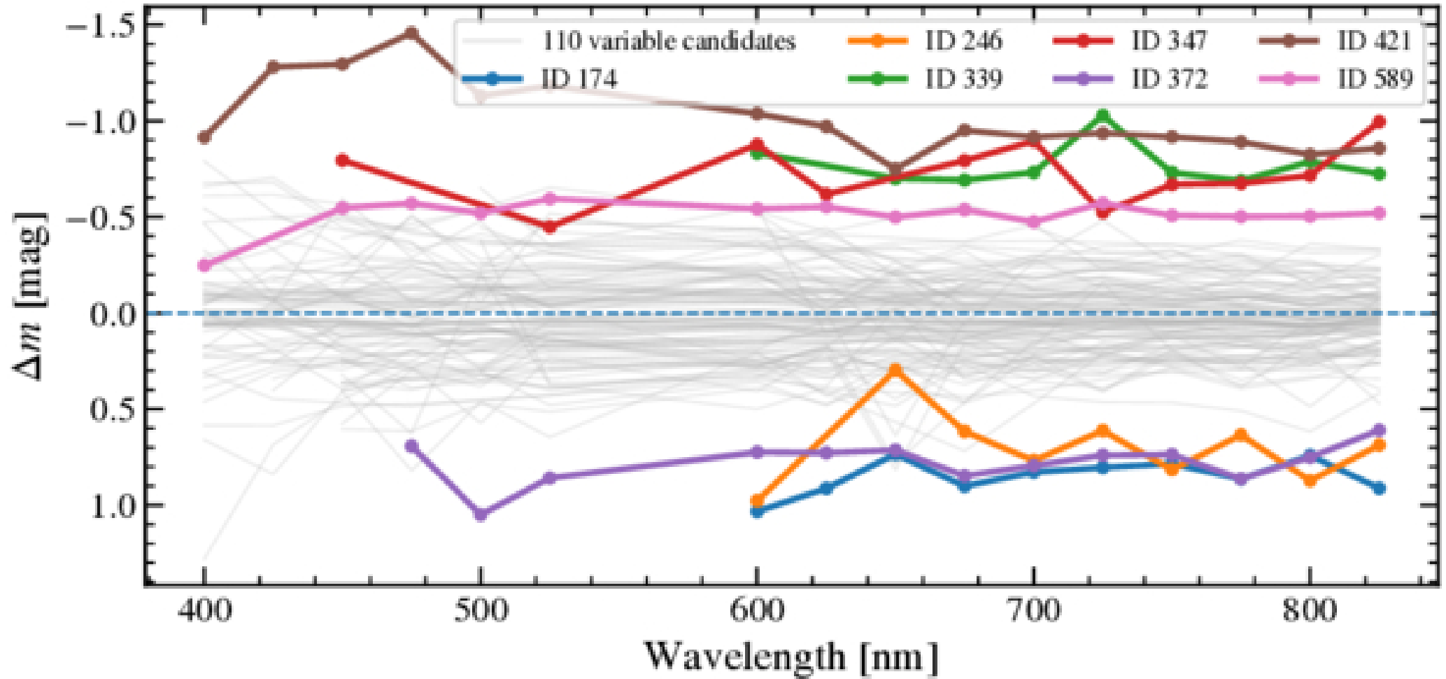
Figure 5. from Mi-Ryang Kim et al 2026 Astron. J. 172 doi:10.3847/1538-3881/ae707f https://dx.doi.org/10.3847/1538-3881/ae707f © 2026. The Author(s). Published by the American Astronomical Society.
