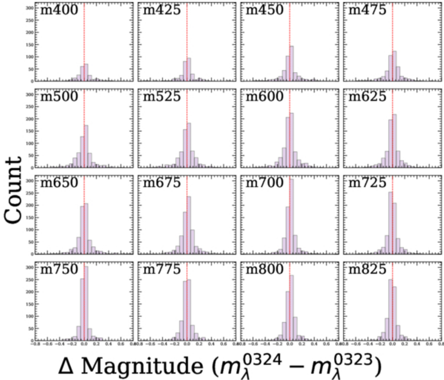
Figure 3. from Mi-Ryang Kim et al 2026 Astron. J. 172 doi:10.3847/1538-3881/ae707f https://dx.doi.org/10.3847/1538-3881/ae707f © 2026. The Author(s). Published by the American Astronomical Society.
