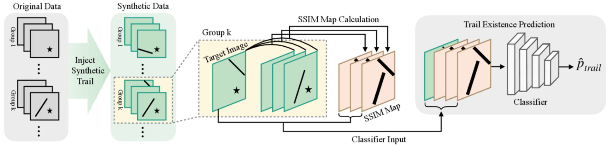
Figure 2. from Mi-Ryang Kim et al 2026 Astron. J. 172 doi:10.3847/1538-3881/ae707f https://dx.doi.org/10.3847/1538-3881/ae707f © 2026. The Author(s). Published by the American Astronomical Society.
