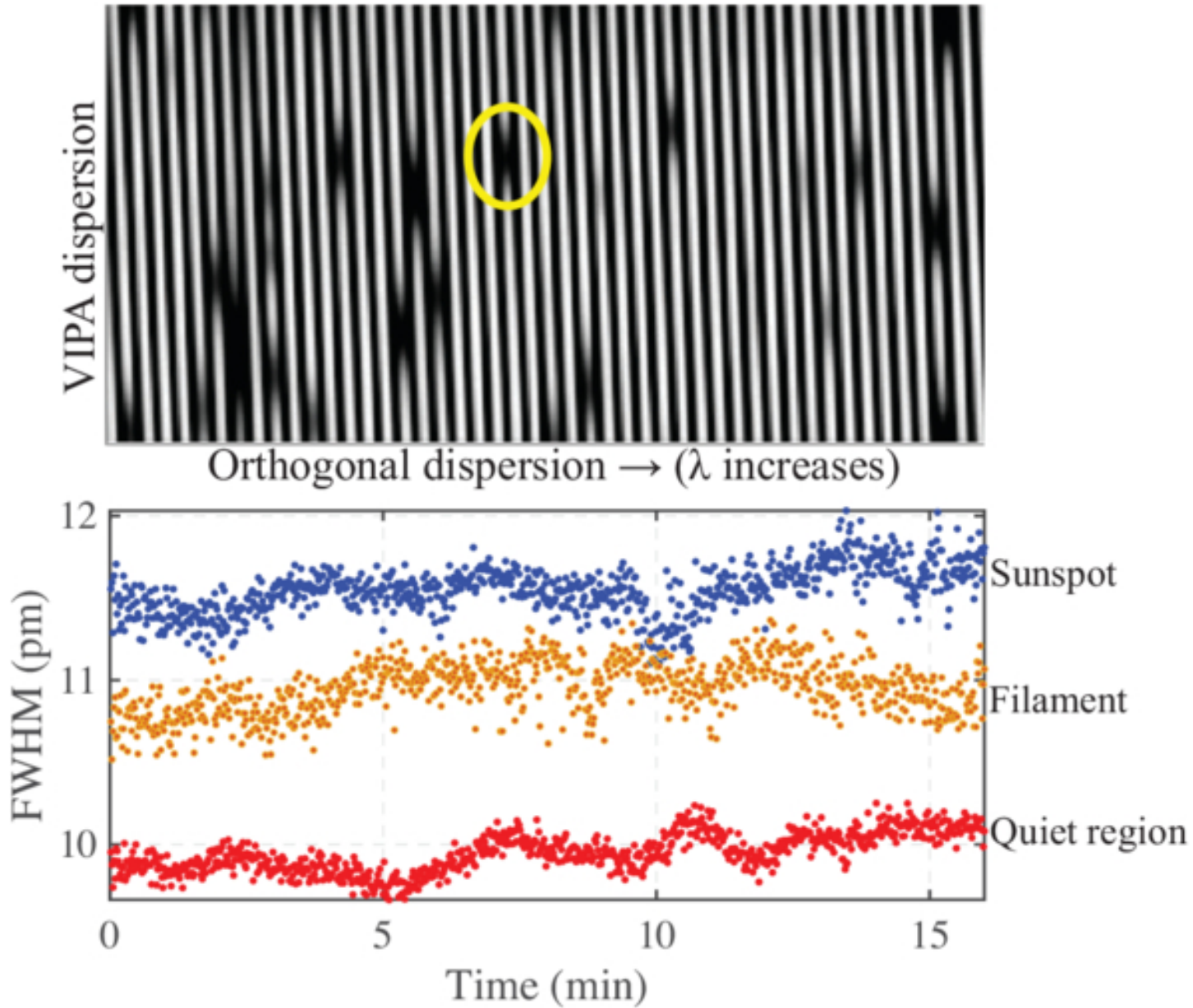
Figure 5. from Yutao Wang et al 2026 Astron. J. 172 doi:10.3847/1538-3881/ae6fb1 https://dx.doi.org/10.3847/1538-3881/ae6fb1 © 2026. The Author(s). Published by the American Astronomical Society.
