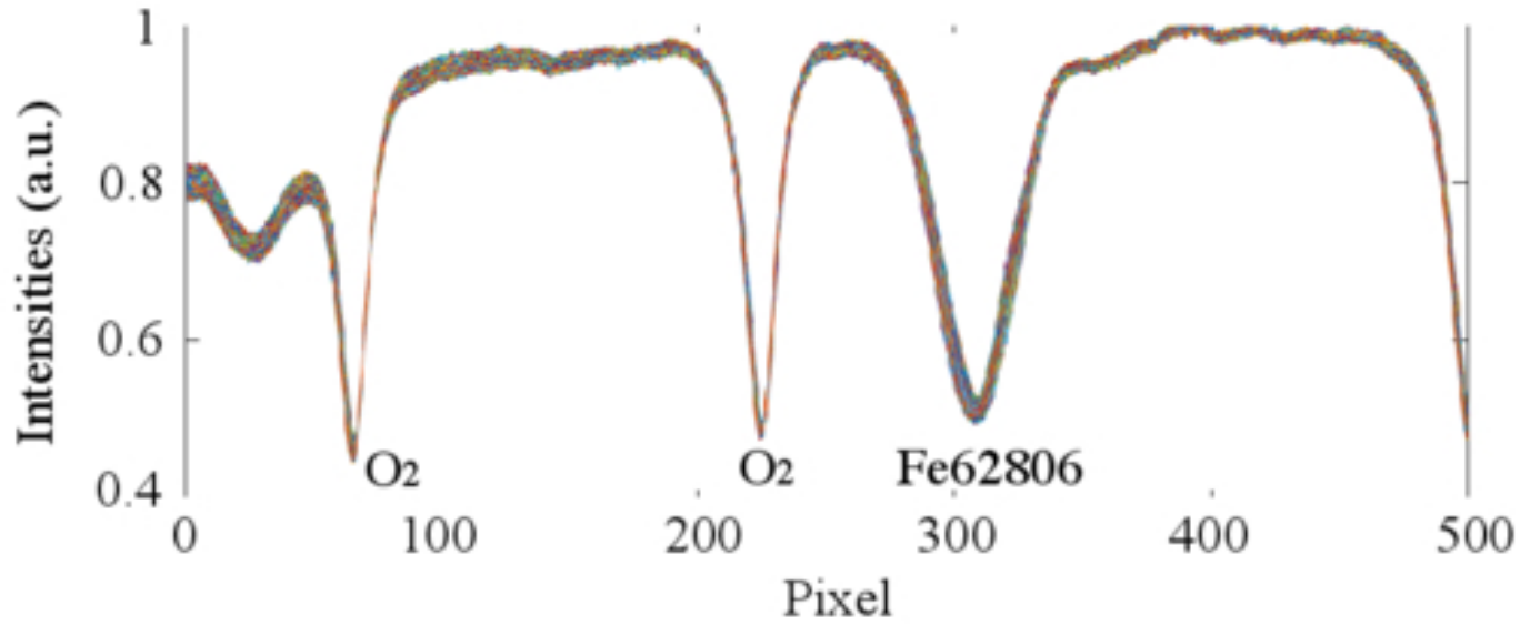
Figure 4. from Yutao Wang et al 2026 Astron. J. 172 doi:10.3847/1538-3881/ae6fb1 https://dx.doi.org/10.3847/1538-3881/ae6fb1 © 2026. The Author(s). Published by the American Astronomical Society.
