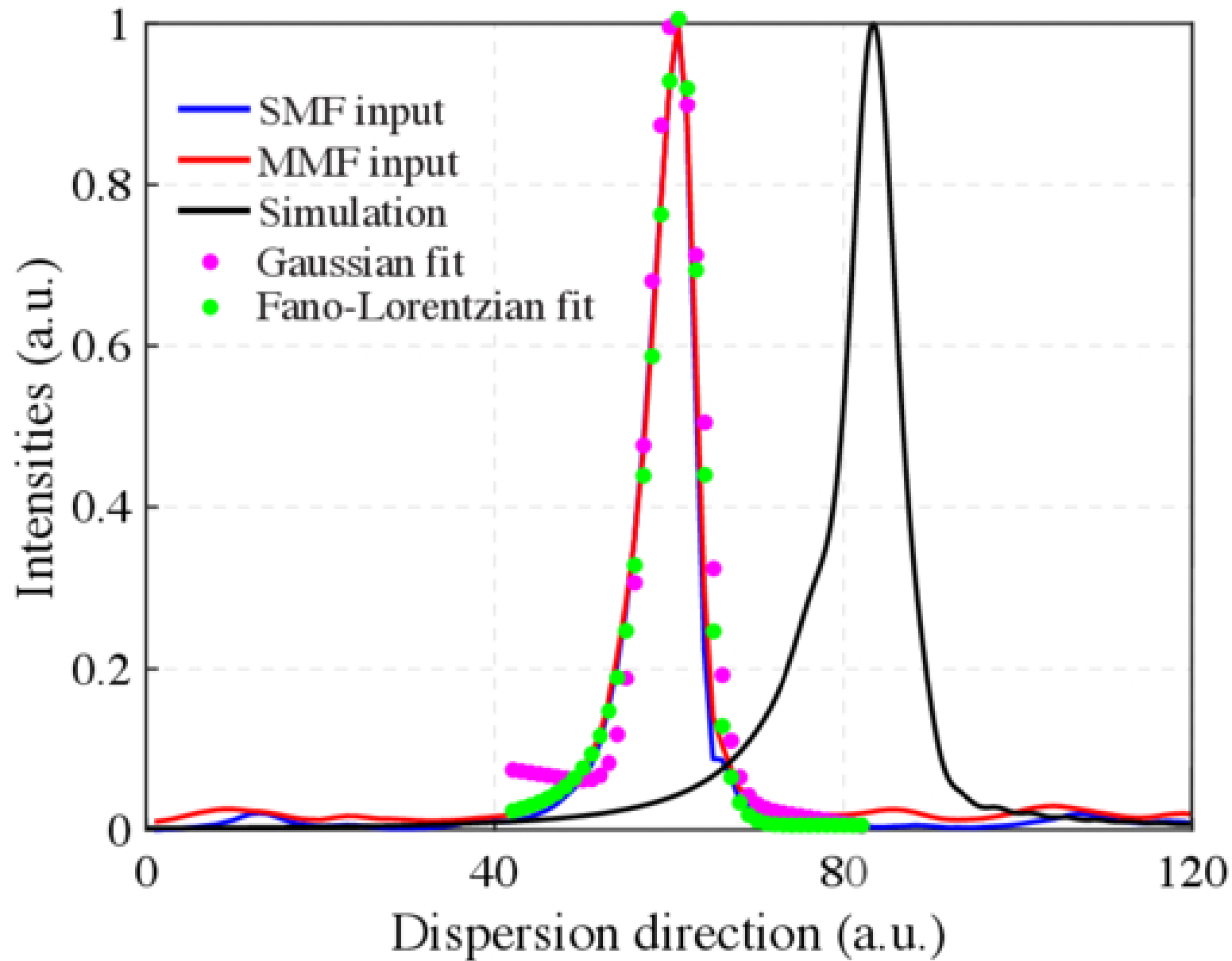
Figure 2. from Yutao Wang et al 2026 Astron. J. 172 doi:10.3847/1538-3881/ae6fb1 https://dx.doi.org/10.3847/1538-3881/ae6fb1 © 2026. The Author(s). Published by the American Astronomical Society.
