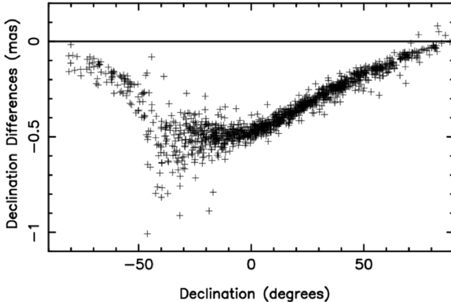
Figure 2. from David Gordon et al 2026 Astron. J. 172 doi:10.3847/1538-3881/ae6efe https://dx.doi.org/10.3847/1538-3881/ae6efe © 2026. The Author(s). Published by the American Astronomical Society.
