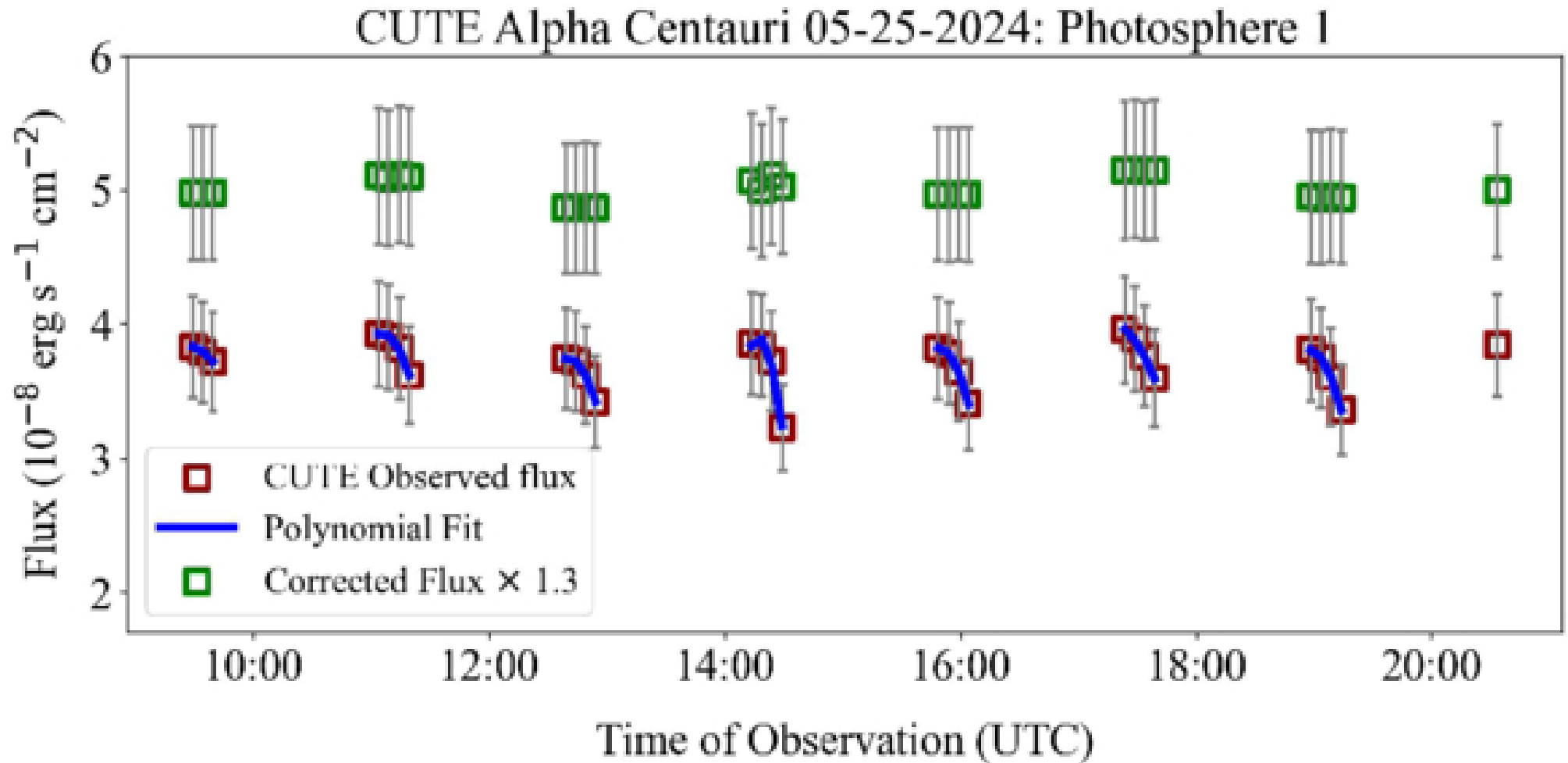
Figure 2. from Dolon Bhattacharyya et al 2026 Astron. J. 172 doi:10.3847/1538-3881/ae6db0 https://dx.doi.org/10.3847/1538-3881/ae6db0 © 2026. The Author(s). Published by the American Astronomical Society.
